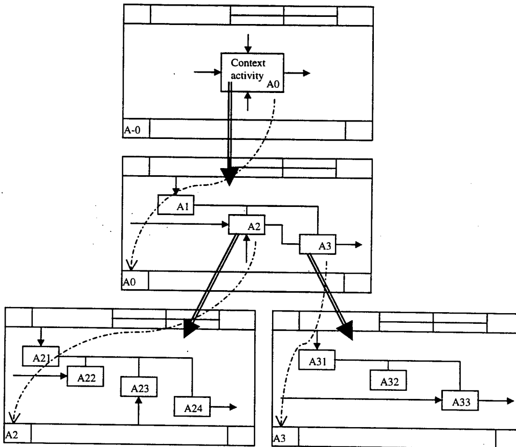
FIGURE 2. A TYPICAL IDEF0 DIAGRAM HIERARCHY
