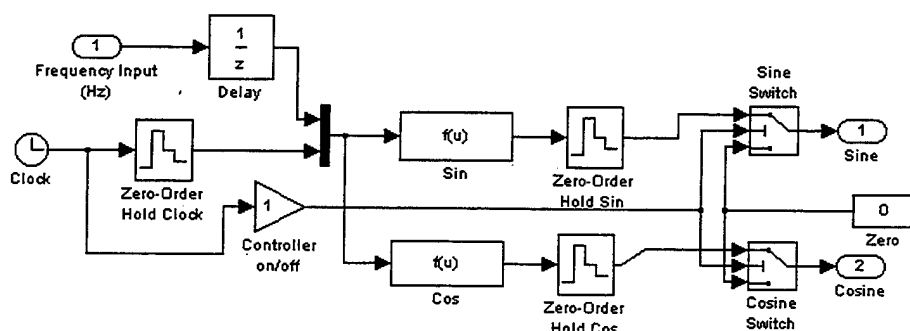
Figure 29. Sine/Cosine Generator
