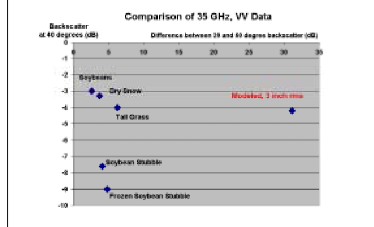
Figure 14. Comparison of modeled and experimental backscatter data.
