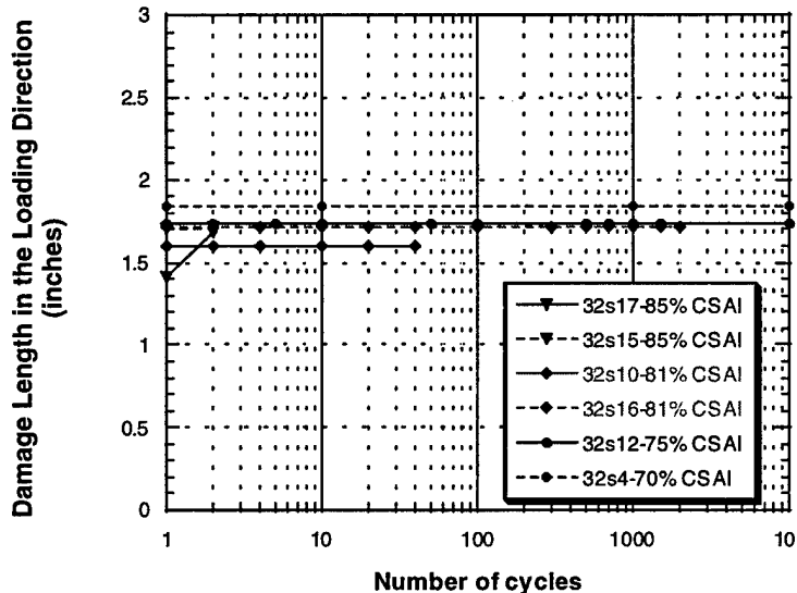
FIGURE 36. DAMAGE GROWTH IN CONSTANT AMPLITUDE COMPRESSION-COMPRESSION LOADING
