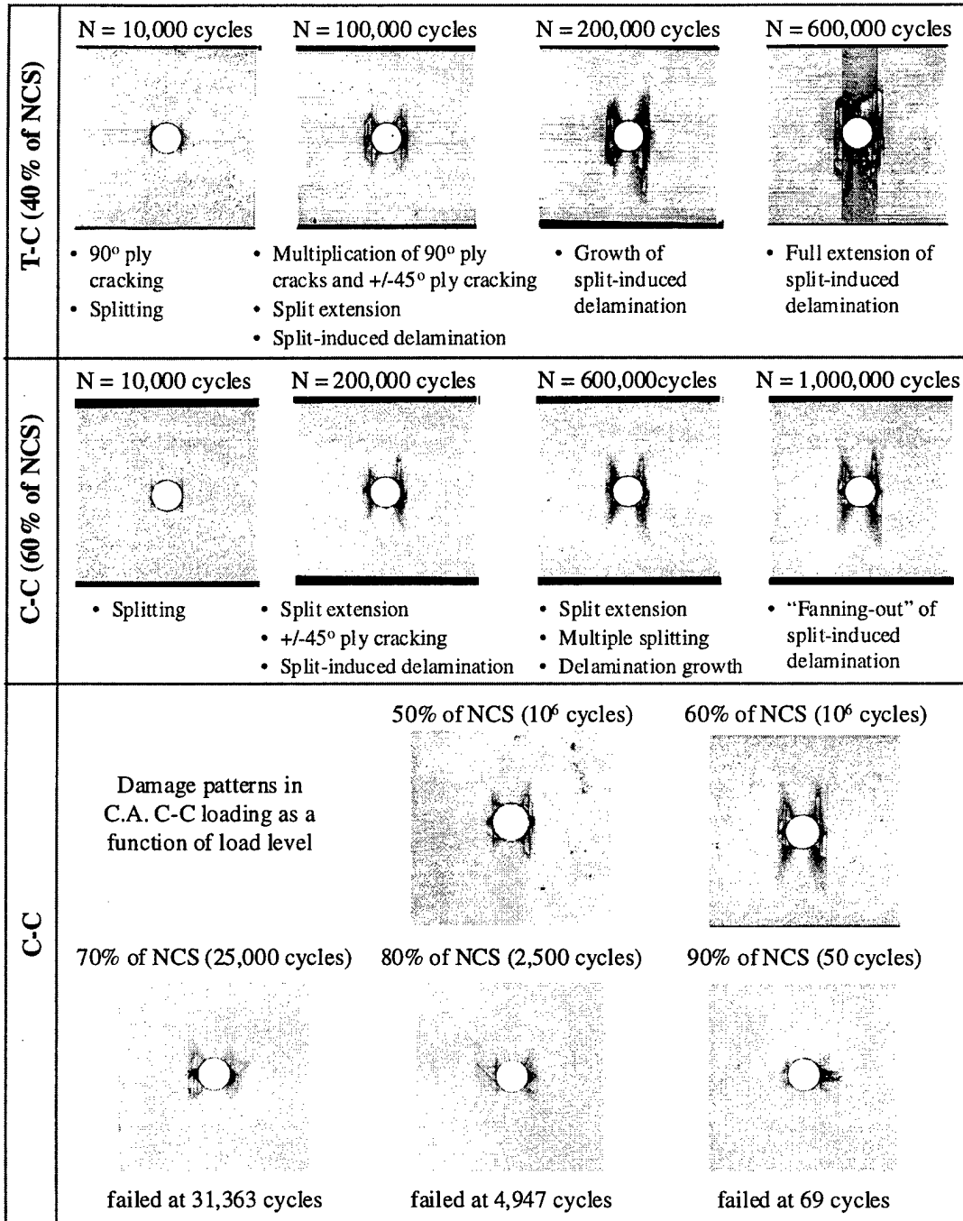
FIGURE 6. DAMAGE ACCUMULATION IN C.A. T-C AND C-C FATIGUE
