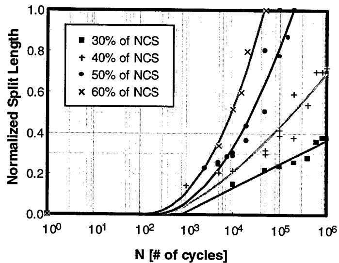
FIGURE 7. NORMALIZED SPLIT LENGTH MEASUREMENT AND NORMALIZED SPLIT LENGTH IN T-C LOADING
