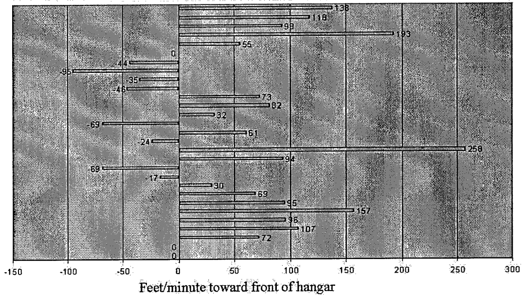
Figure 6. Air Movement at the Leading Edge of the Wings of a B-1B Aircraft in Building 198 Before (Upper) and After (Lower) Three Iterations of Adjustments to Orientation of Exit Ducts and Louvers.
