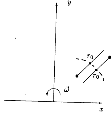
Figure 2: Radial Relative Equilibrium Configurations
