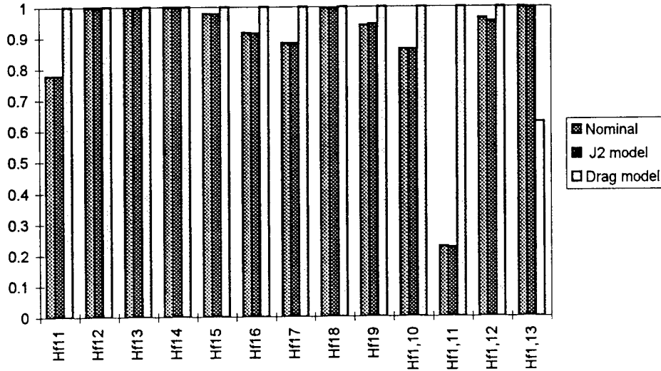
Fig. 2. Effect of Oblateness and Drag on Magnitude of each Element of \mathbf{H}_f Matrix. (Range observations for 1/16^{\text{th}} period. Estimation vector \mathbf{x} = [r \ \Omega \ i \ \theta \ \theta_2 \ \theta_3 \ \dot{r} \ \lambda_3 \ \omega_2 \ \omega_3 \ m \ m_p \ \rho] )
