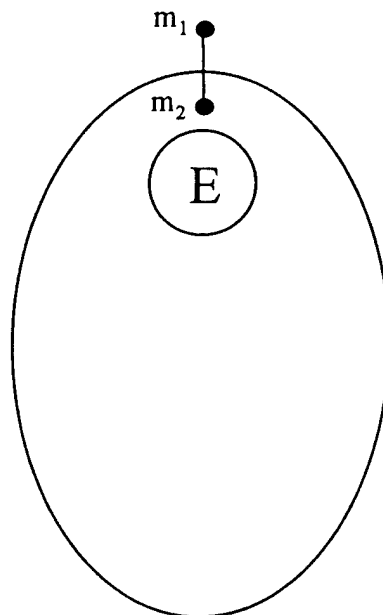
Figure 5. Center of Mass in an Elliptical Orbit at Perigee, no Libration.
