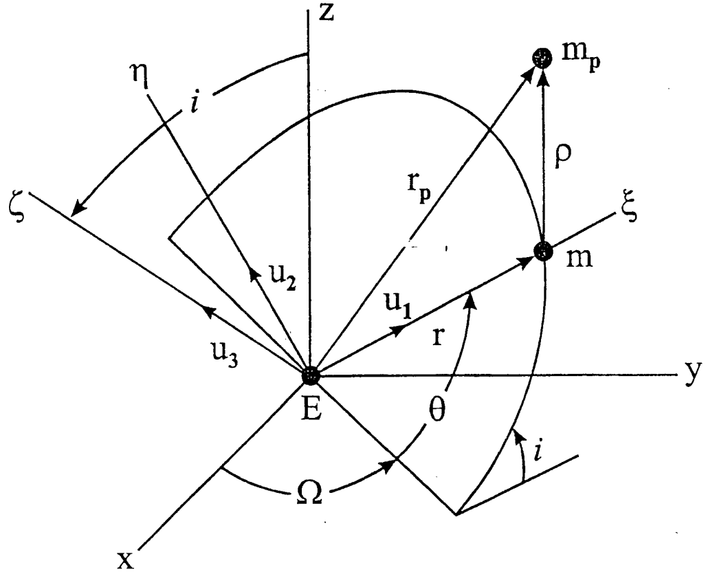
Figure 1. Osculating Orbit Plane.
