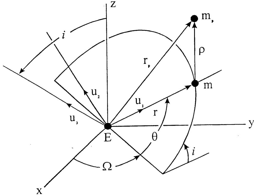
Figure 1. Osculating Orbit Plane
