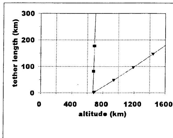
Figure 8. Delineation Between Areas of Actual Re-entry, Apparent Re-entry, and No Re-entry.
