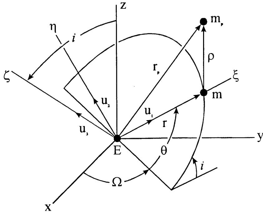
Fig. 1a. Osculating Orbit Plane ( u_1, u_2, u_3 ).
