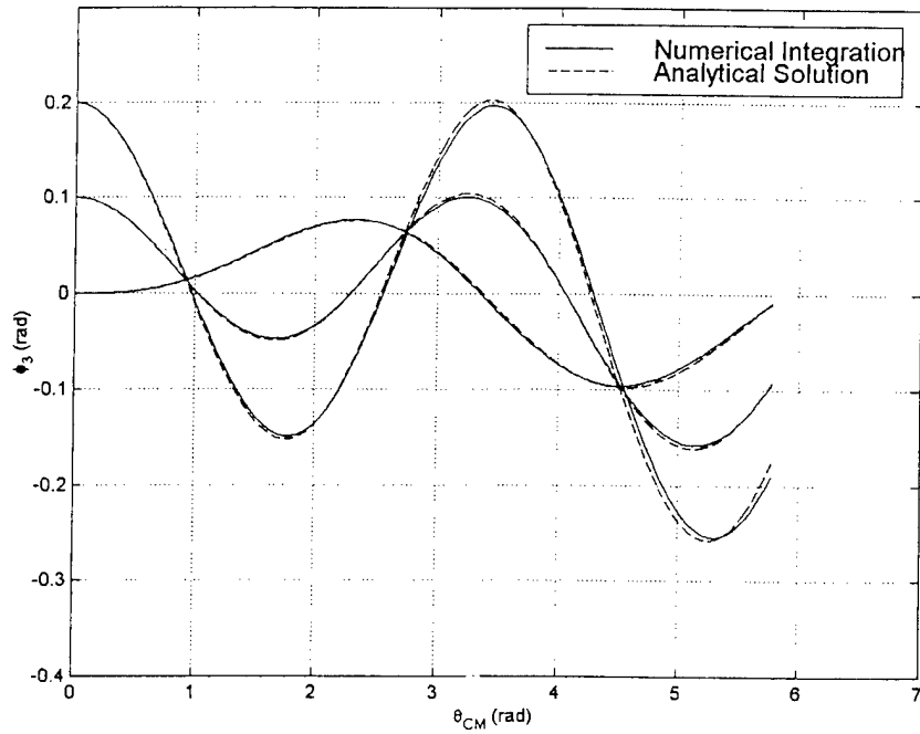
Fig. 9. Comparison of Analytical and Numerical Results. (Tether Length=10 km and m / m_p = 1.0 )
