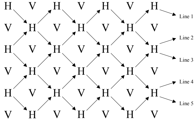
Figure 4. Schematic diagram of the readout scheme. H and V represent pixels sensitive to horizontally-polarized and vertically-polarized infrared radiation, respectively.
