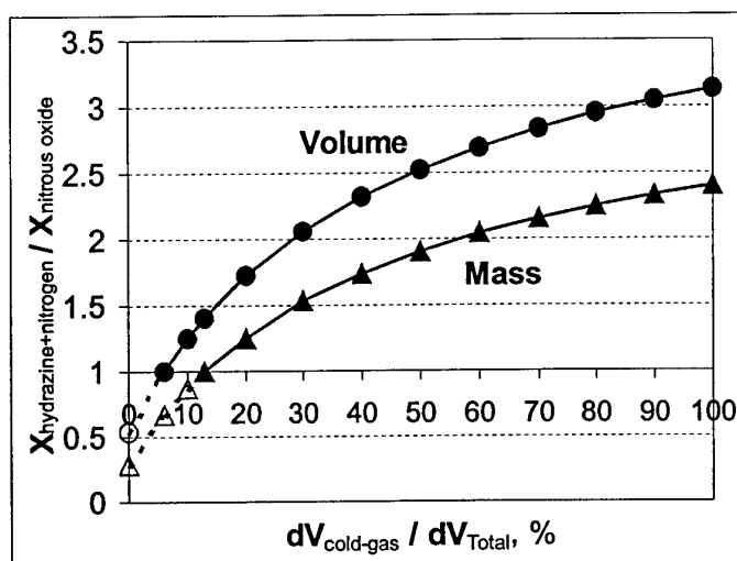
Fig. 9: Performance comparison of hydrazine monopropellant/nitrogen cold-gas to nitrous oxide monopropellant/cold-gas dual-mode propulsion. ( dV – spacecraft velocity change; X denotes propulsion mass or volume respectively)
