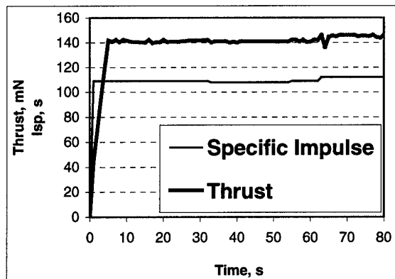
Fig. 6: Thrust and specific impulse for UoSAT-12 resistojets firing on 11 April 2000.
