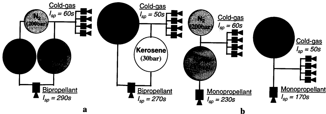
Fig. 16: Schematics of dual-mode propulsion system options for small satellite: a) Cold-Gas/Bipropellant; b) Cold-Gas/ Monopropellant.
