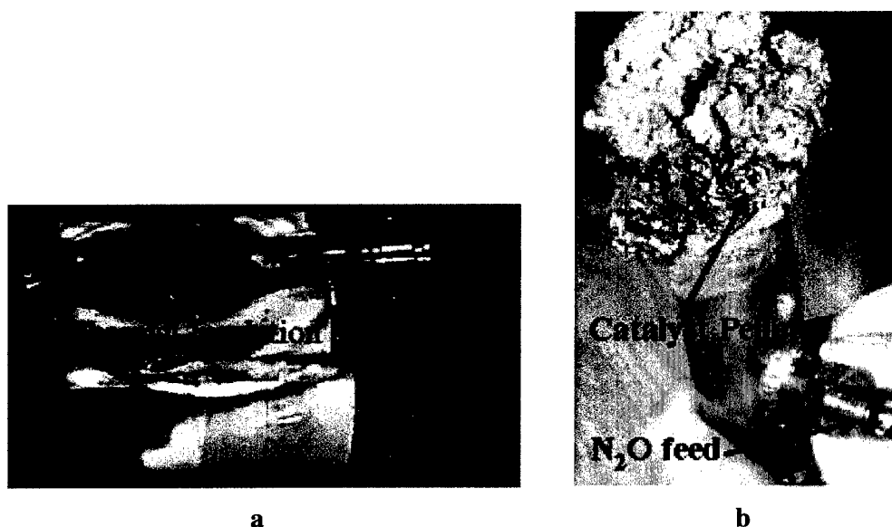
Fig. 34: Test design after firing: a) Stainless steel pipe is melted with iron catalyst and MICROPORE thermal insulation; b) Alumina pellets coated by catalyst have survived the heat.
