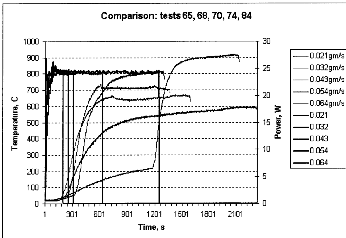
Fig. 27: Exhaust gas flow temperature of decomposition reaction products and electric power input as a function time.
