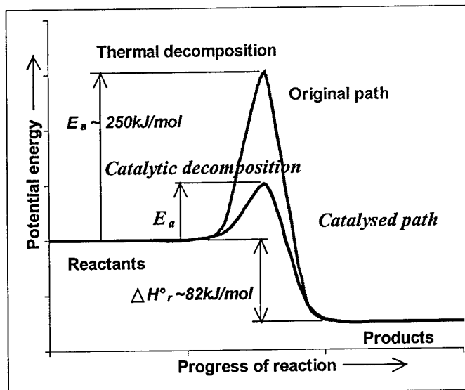
Figure 1. Nitrous oxide decomposition. ( E_a – activation energy; \Delta H^\circ – reaction enthalpy)
