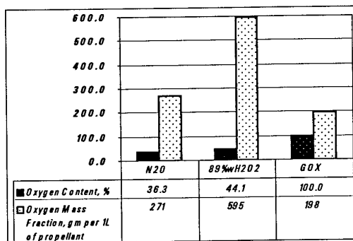
Figure 4 Amount of free oxygen available for combustion.
