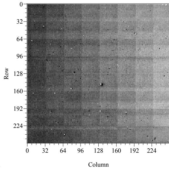
Figure 8. Histogram (a) and grayscale image (b) of the conversion efficiency (quantum efficiency-gain product) for the LWIR part of the FPA.
