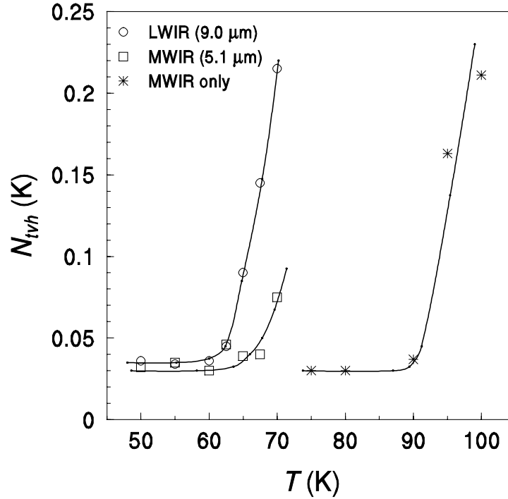
Figure 10. Mean temporal NE \Delta T ( N_{tvh} ) as a function of operating temperature for the dual-band FPA. The circles and squares are the values of NE \Delta T measured when operating conditions were optimized for running both bands simultaneously, the stars show the values of NE \Delta T measured when the conditions were optimized for the MWIR array alone. The lines are simply guides to the eye.
