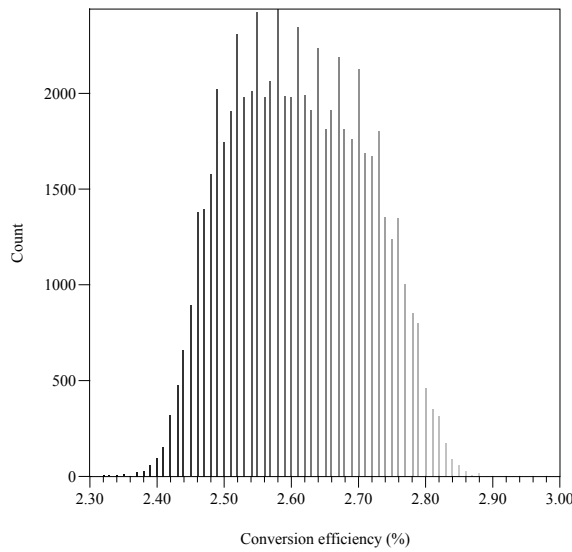
Figure 8. Histogram (a) and grayscale image (b) of the conversion efficiency (quantum efficiency-gain product) for the LWIR part of the FPA.
