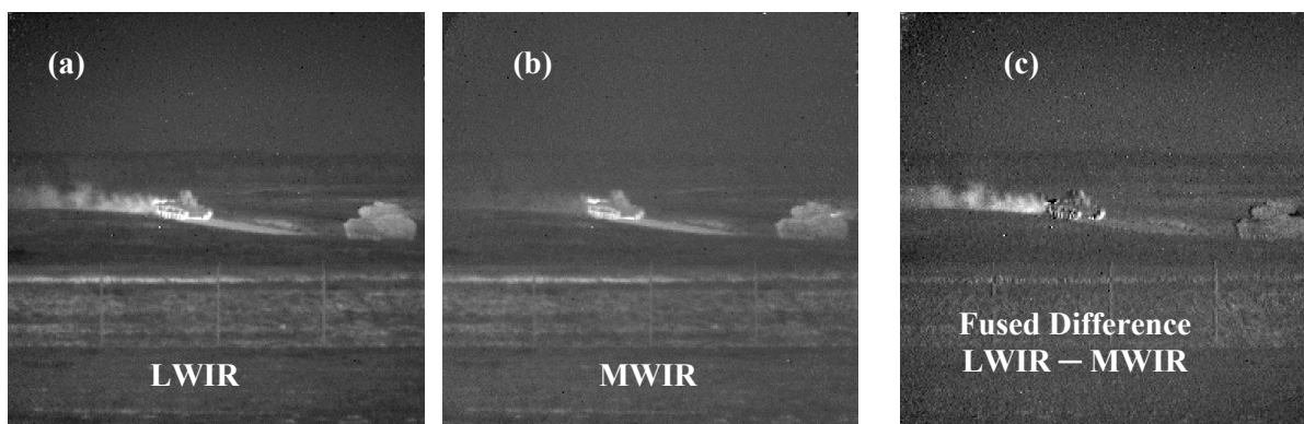
Figure 13. Simultaneous dual-band image of an M60 tank and an M2 Bradley fighting vehicle. The LWIR image (a) clearly shows a dust plume behind the tank that is barely visible in the MWIR image (b). In the MWIR image, the engine exhaust of the M2 can be seen more clearly than in the LWIR image. The fused difference image (LWIR - MWIR) is shown in (c); objects with large LWIR signatures (relative to MWIR) are bright and those with large MWIR signatures are dark.
