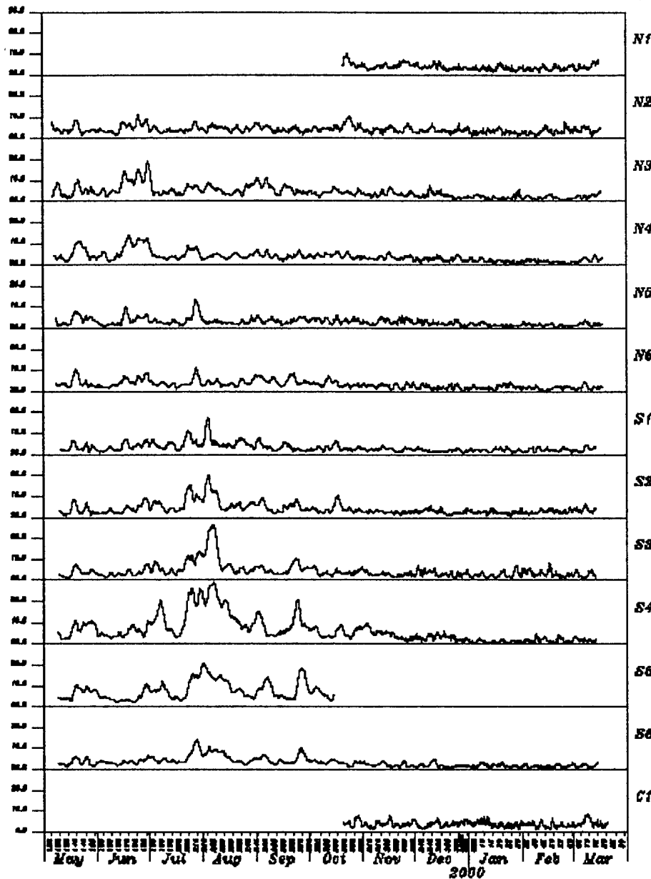
Figure 2. The vertically averaged amplitude of the negative rotary spectra at only the inertial frequency for the 13 ADCP moorings indicates the main events occur in May through September. Very little variability occurs at the inertial frequency during winter. The variability in the southern line during July/August is correlated to the passage of a typhoon event traveling northeast and passing across Kyushu (see wind stress curl in Figure 6).
