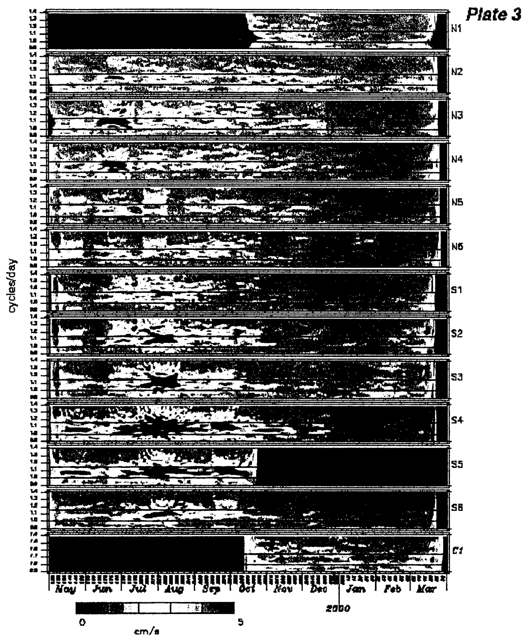
Plate 3. The time-varying amplitude spectra using a 20 day window indicates the frequency at which the energy is occurring. The 20 day window provides a frequency resolution of 0.05 cpd. The two horizontal lines in each plot are at the 1 cpd and 1.15 cpd frequencies. Most of the energy is at a frequency slightly less than the inertial.
