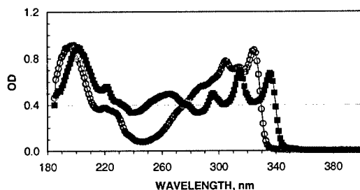
Fig.5. Measured optical density of PTPT-35 (gray) and PTTP-24 (black). Concentration=1%, d=6\mu\text{m} , and host ZLI-2359.
