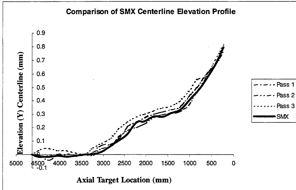
Figure 5. Comparison of Optical Measurement Technique to SMX Method.
