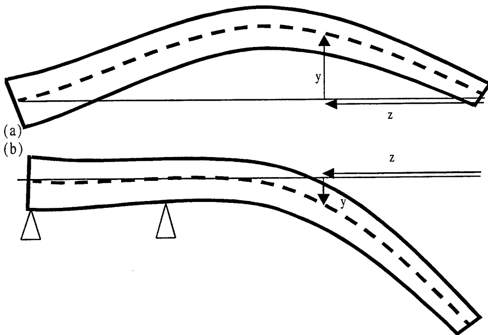
Figure 1. Two Methods of Specifying Barrel Curvature: (a) Relative to a Line Through the First and Last Bore Center Measurements, or (b) Relative to a Line Through the Bore Center at its Support Points.
