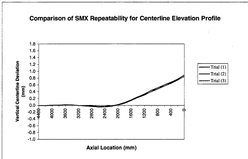
Figure 6. Comparison of Repeatability of SMX Method.
