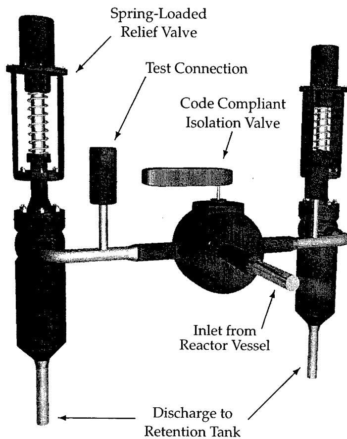
Figure 7-3: Redundant Spring-Loaded Relief Valves with ASME Boiler and Pressure Vessel Code Compliant Isolation
