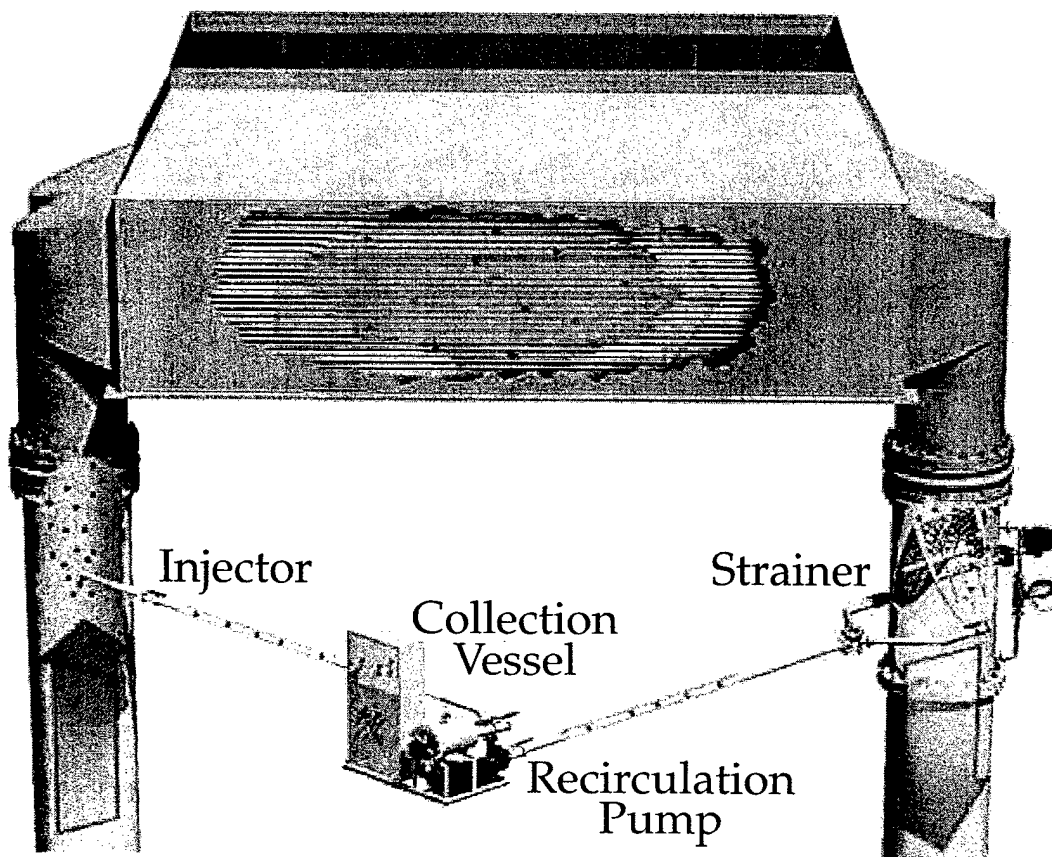
Figure 9-2: Ball-Type On-Line Condenser Cleaning System Operation. Abrasive balls are pumped from the collection vessel to the injector, where they enter the condenser waterbox inlet head. After passing through a random tube, the balls are captured by the strainer and directed (via the recirculation pump) to the collection vessel.
