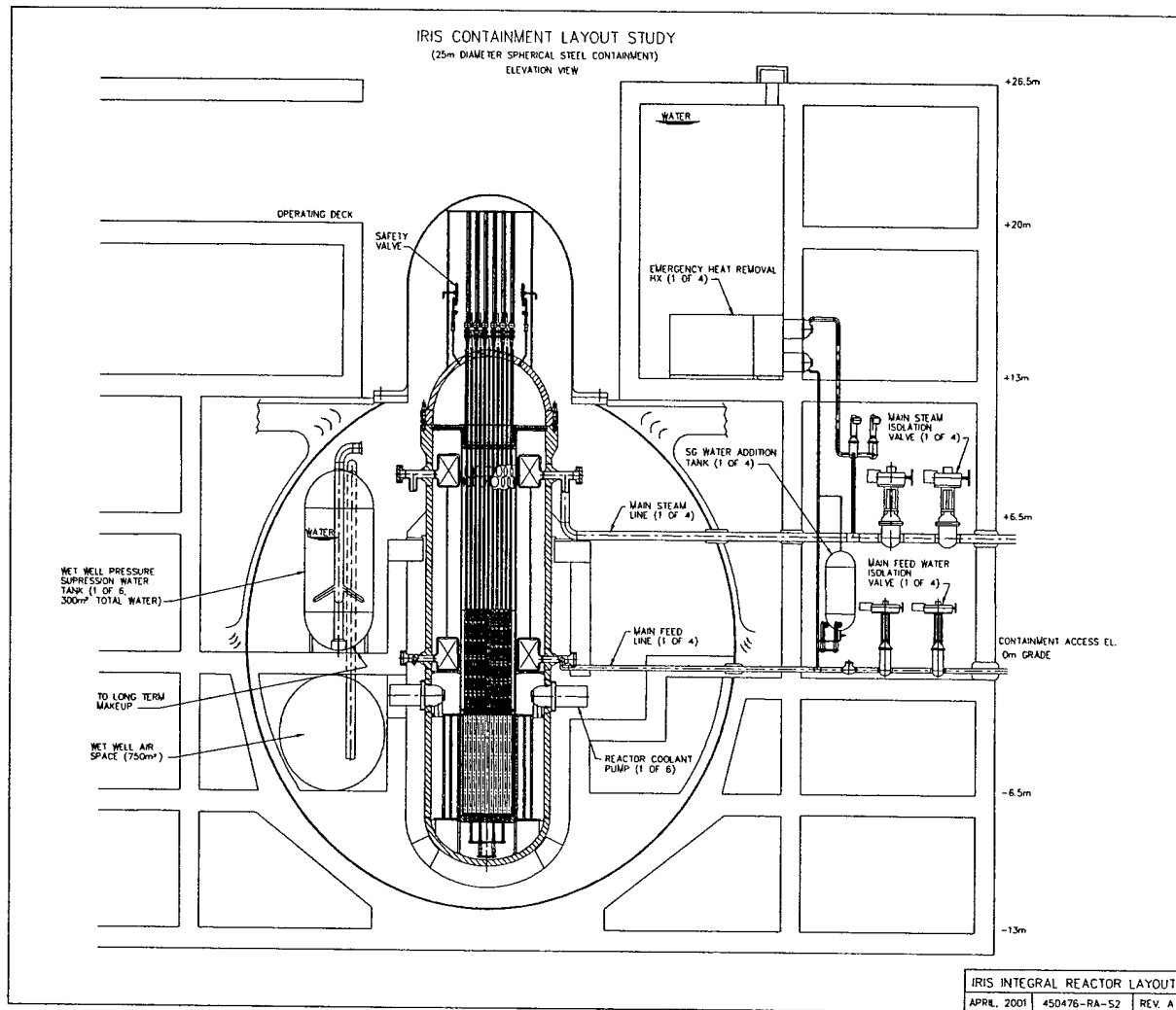
Figure 6-1: IRIS Containment Arrangement Showing Passive Cooling Loop (1 of 4 loops shown)
