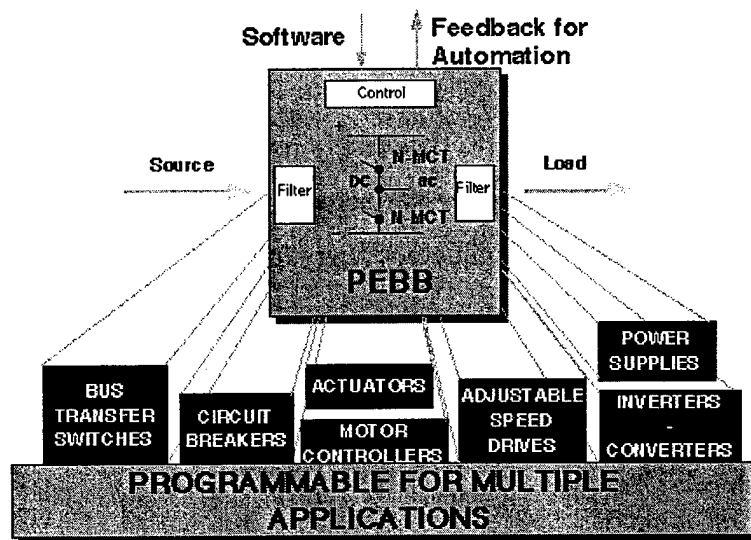
Figure 4-2: Power Electronics Building Block Functional Diagram
