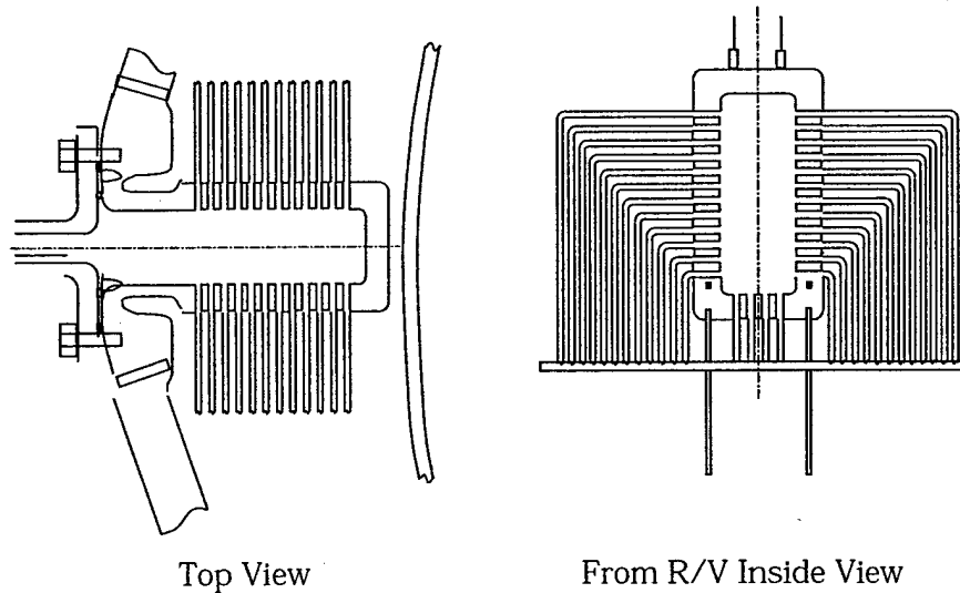
Figure 8-2: Conceptual Drawing of IRIS C-Tube Steam Generator
