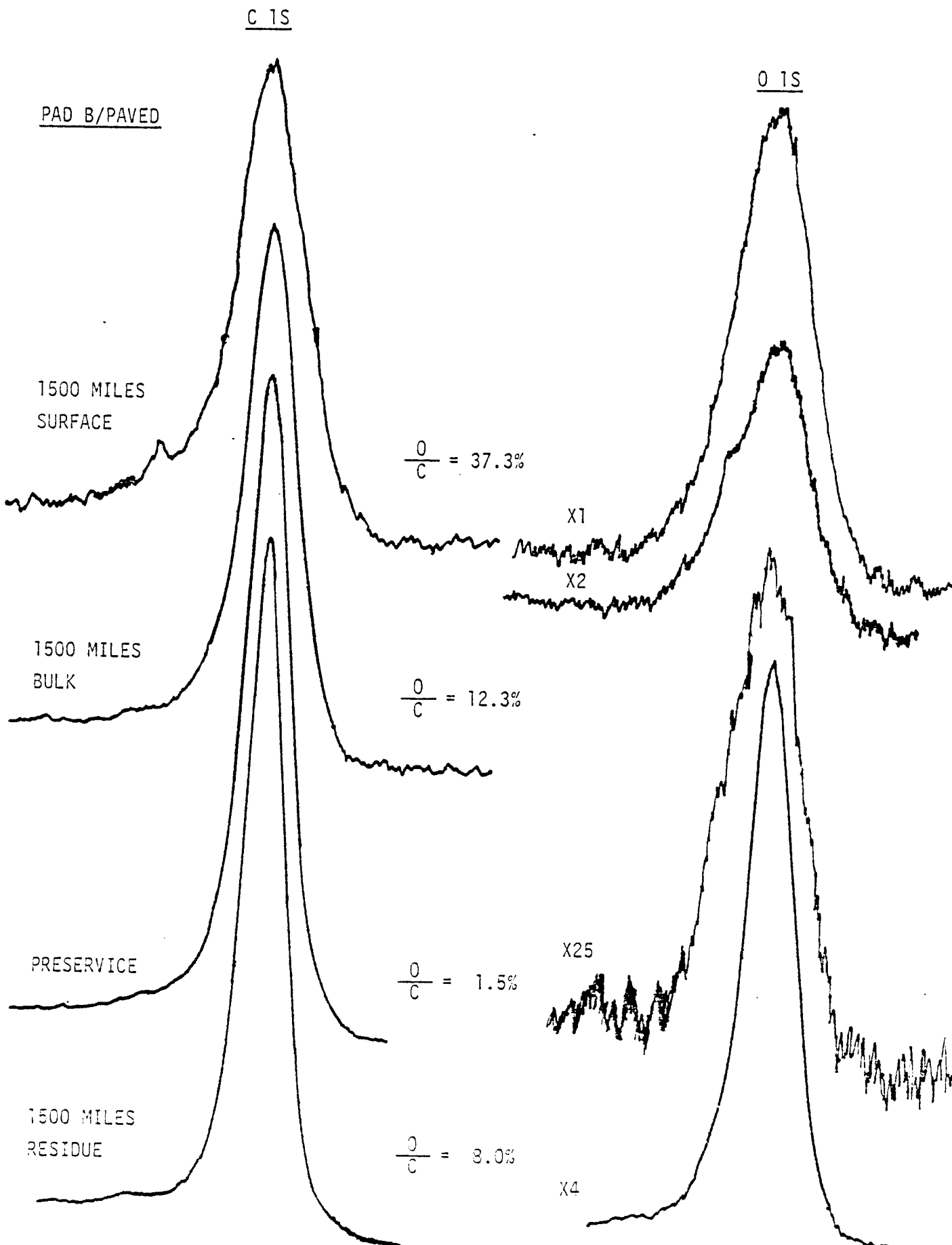
Figure 4. Comparison of Carbon and Oxygen 1s ESCA Spectra for Firestone Pad
