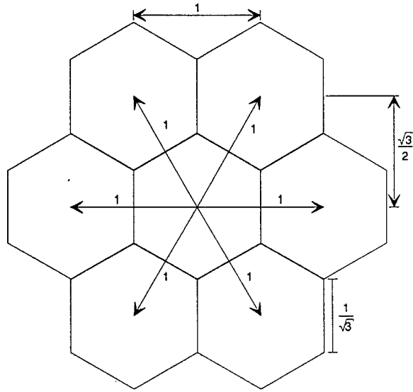
Figure 3.3 Regular Hexagonal Pixel Geometry.
