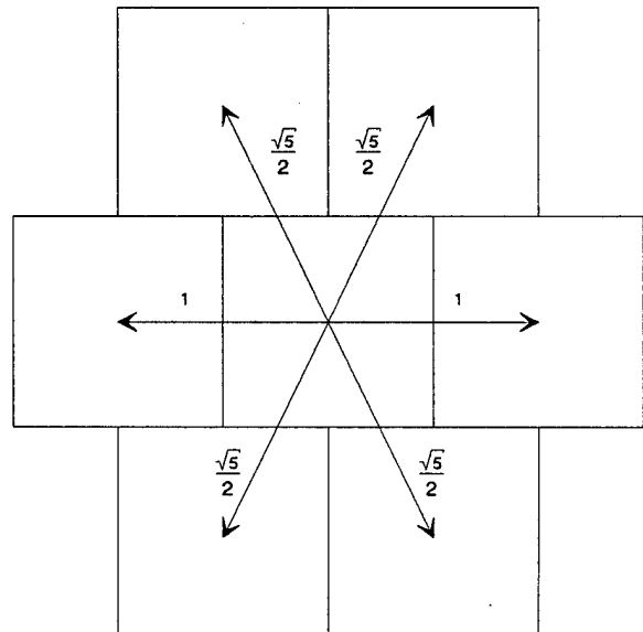
Figure 3.4 Staggered Square Pixel Geometry.
