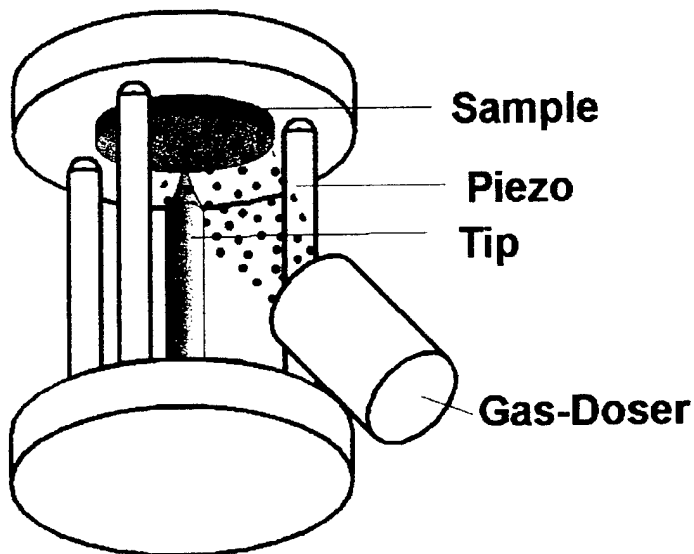
Figure 15: Schematic of experimental set-up for STM assisted growth of Ge dot.
