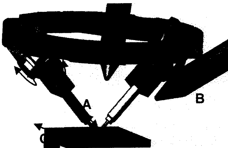
Figure 12. Up to four independently working STMs (A) are combined in the nanoworkbench. They will be used to create patterns of carbon or Sb atoms on the Si substrate. Evaporators(B) allow parallel deposition of Germanium and Si material. A high precision sample translation stage allows large scale positioning in x/y directions of the silicon substrate (C).
