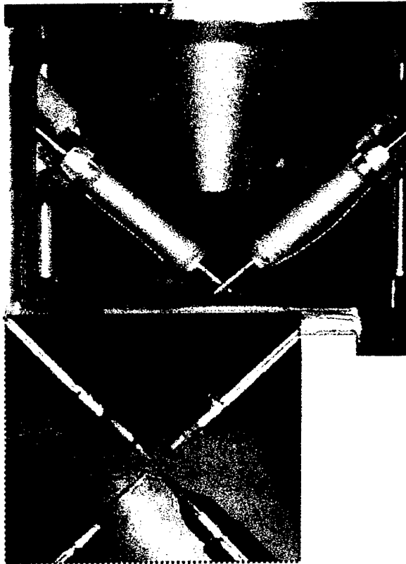
Figure 9. The electron column mounted in the UHV chamber (only the exit end is seen) together with the two STM tips, approaching each other.
