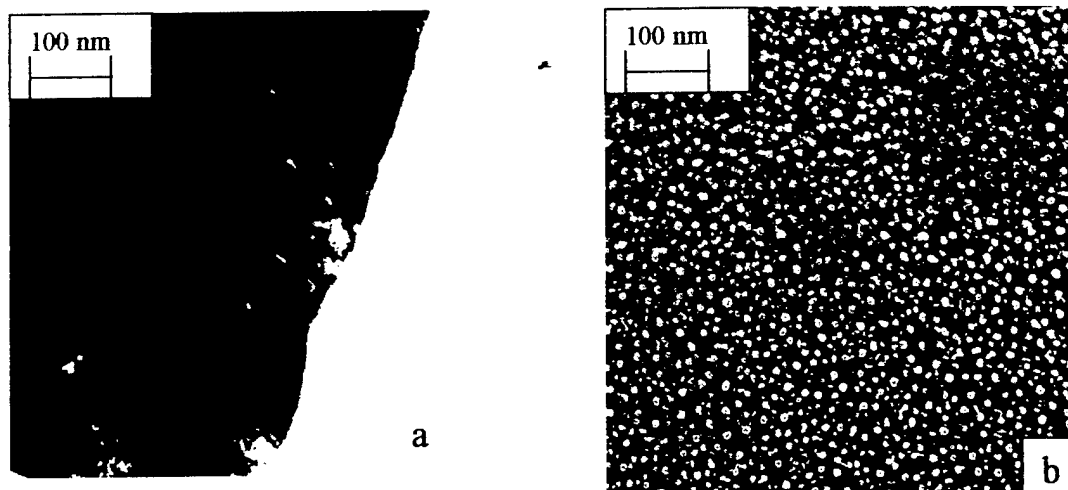
Figure 16: (a) Free-standing single carbon nanotubes grown on Ni catalysts deposited on a Cu substrate. (b) Uniformly-sized Ni particles grown on a Si(110) substrate.
