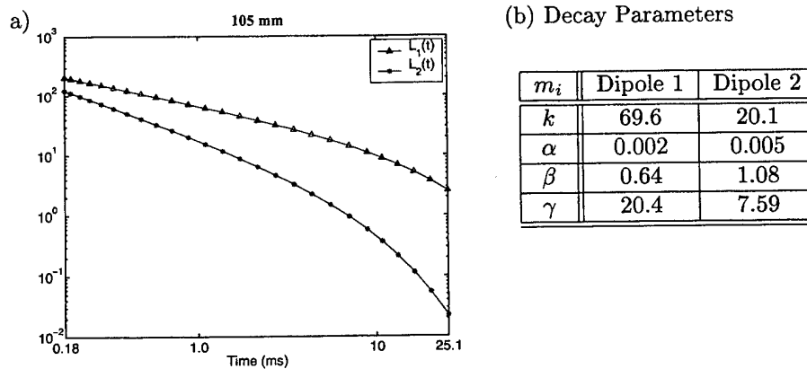
Figure 51: 105 mm Projectile
