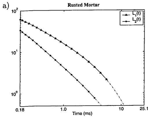
Figure 53: Rusted Mortar
