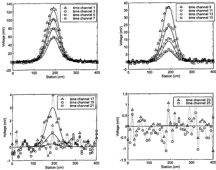
Figure 22: 60mm Mortar: \theta = 0 degrees (vertical), Z = 73 cm.
