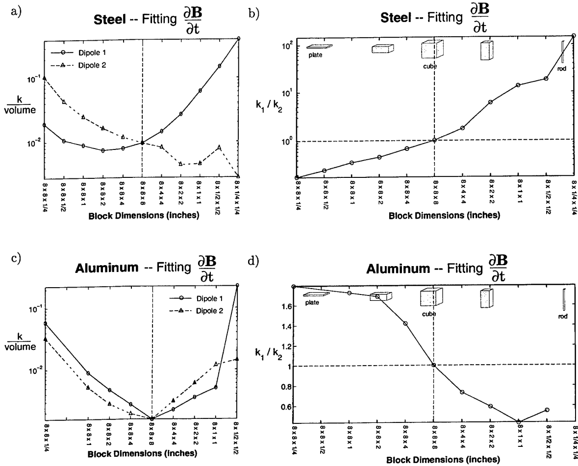
Figure 5: Relating the aspect ratio of a steel target with the ratio k_1/k_2 . Plot (a) contains the recovered k parameter from fitting the measured \partial B/\partial t response of steel axi-symmetric targets. Plot (b) illustrates the relationship between the k_1/k_2 ratio derived from the measured \partial B/\partial t response and the shape of a steel target. Plot (c) contains the recovered k parameter from fitting the measured \partial B/\partial t response of aluminum axi-symmetric targets. Plot (d) illustrates the relationship between the k_1/k_2 ratio and the shape of an aluminum target.
