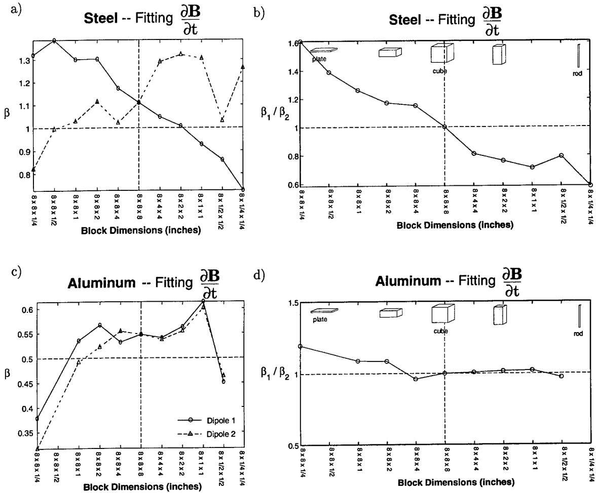
Figure 6: Relating the aspect ratio of a steel target with the ratio \beta_1/\beta_2 . Plot (a) contains the recovered \beta parameter from fitting the measured \partial B/\partial t response of steel axi-symmetric targets. Plot (b) illustrates the relationship between the \beta_1/\beta_2 ratio derived from \partial B/\partial t data and the shape of a steel target. Plot (c) contains the recovered \beta parameter from fitting the measured \partial B/\partial t response of aluminum axi-symmetric targets. Plot (d) illustrates the relationship between the \beta_1/\beta_2 ratio and the shape of an aluminum target.
