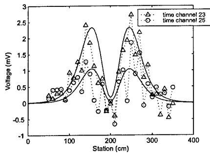
Figure 29: Stokes Mortar: \theta = 90 degrees (horizontal), Z = 73 cm.
