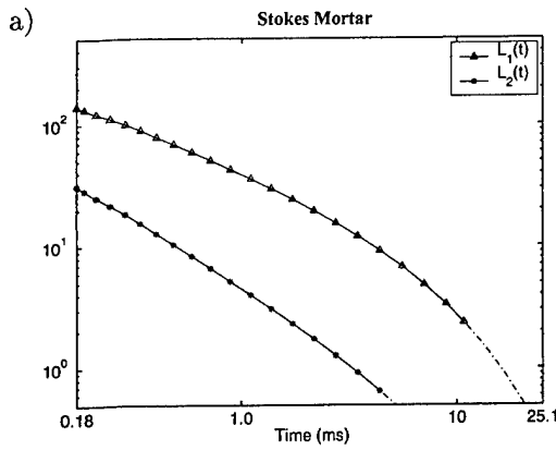
Figure 52: Stokes Mortar
