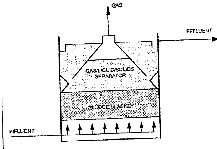
Figure 11: Schematic Representation of an Upflow Anaerobic Sludge Blanket Reactor (UASB) Source: McLean 1995
