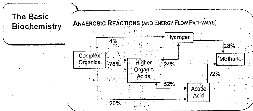
Figure 9: Anaerobic Reactions and Energy Flow Pathways Source: EFX Systems Inc. 1999
