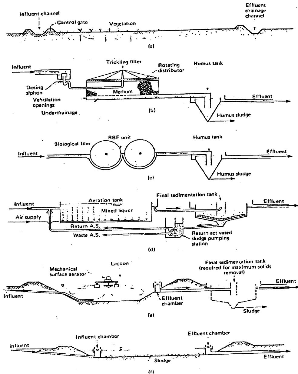
Figure 7: Diagrams of the Principal Biological Treatment Systems: (a) Land Treatment, (b) Tricking Filter, (c) Rotating Biological Filter, (d) Activated Sludge, (e) Aeration Lagoon, (f) Waste Stabilization (Oxidation) Pond Source: Barnes 1995
