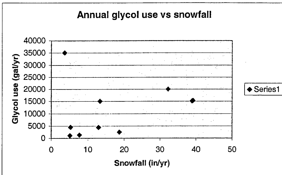
Figure 15: Average Annual Glycol Use at Various Air Force Bases versus Snowfall
