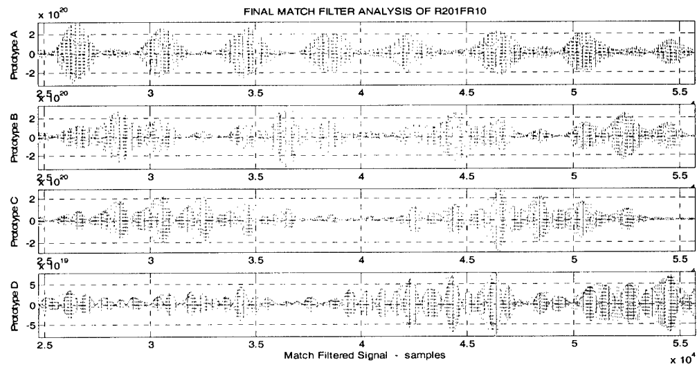
Figure 5.11b. Unresolvable Message Using MESS Approach Transmitted in a Noisy Environment ( SNR_A = -1.8 dB, SNR_B = 3.4 dB, SNR_C = 0.8 dB, and SNR_D = 1.4 dB).
