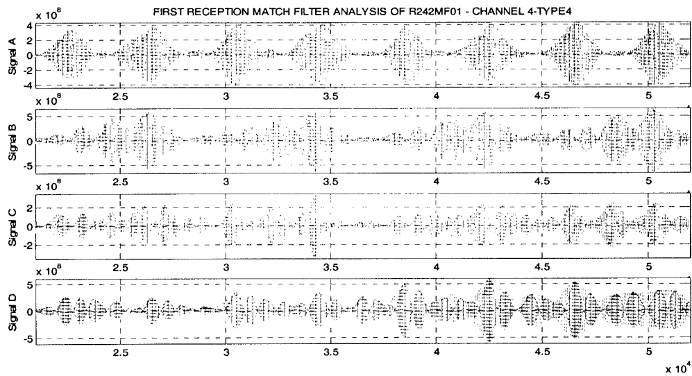
Figure 5.12b. Resolvable Message Using TRAC Approach Transmitted in a Noisy Environment ( SNR_A=13.6 dB, SNR_B=17 dB, SNR_C=10.5 dB, and SNR_D=7.4 dB).
