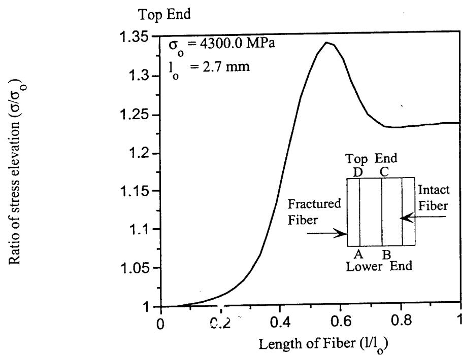
Figure 7.15: stress debonding vf 35
