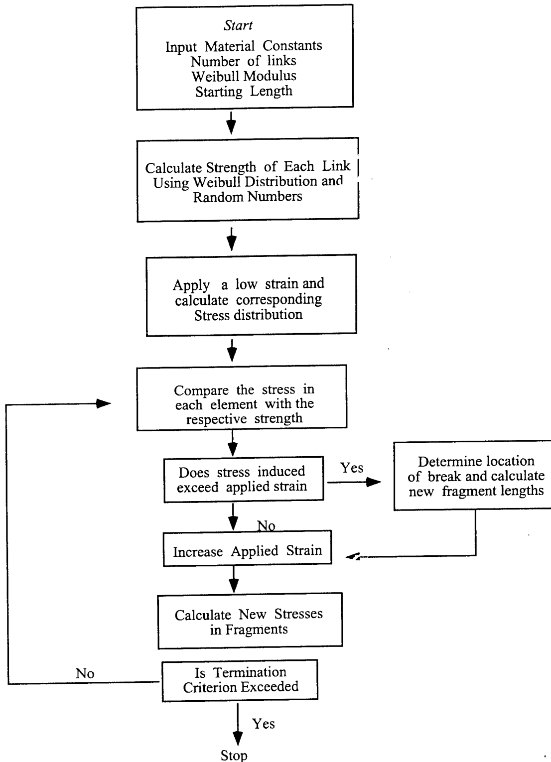
Figure 8.3: Flow chart for the simulation of the fiber fragmentation test
