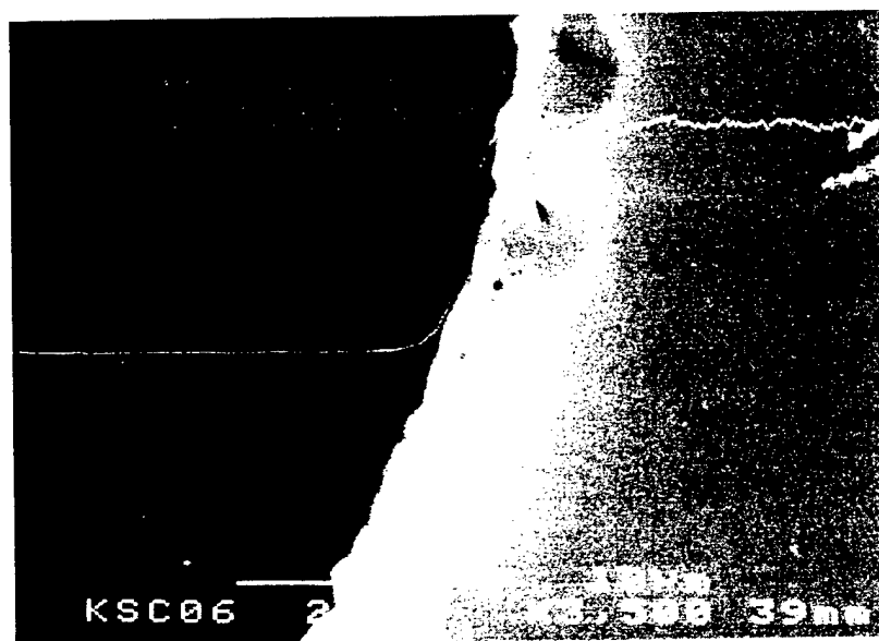
Figure 3.6: Titanium x-ray scan of a SCS-6/Timetal 21s specimen exposed to 927° C for 120 hours (a) line scan (b) dot map
