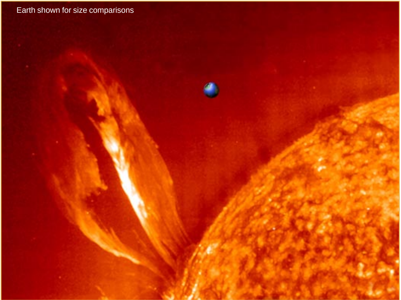
Electromagnetic Radiation
