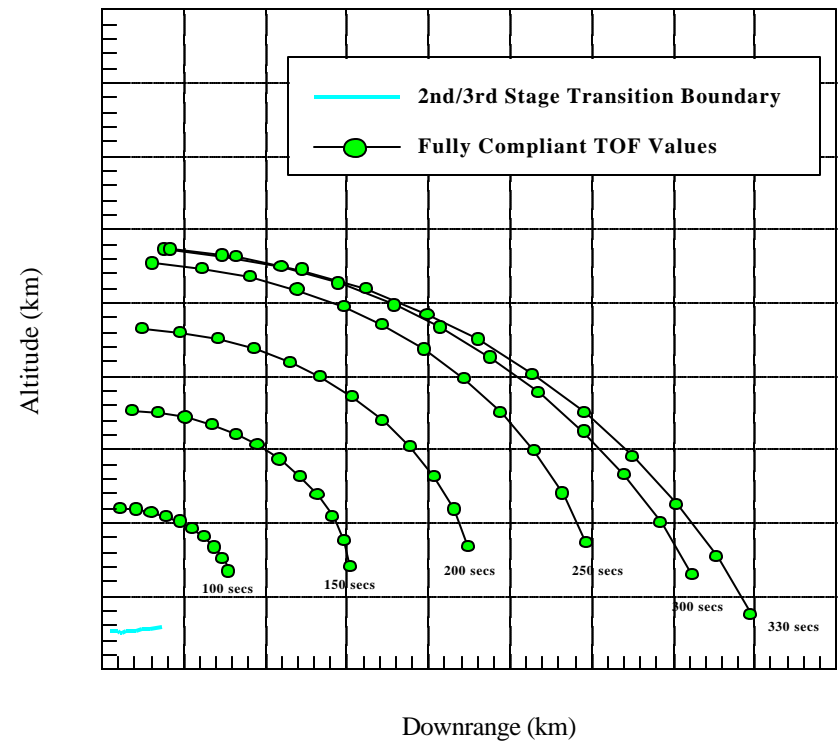
Fan of Trajectories for Varying Injection Angles and Flight Times
