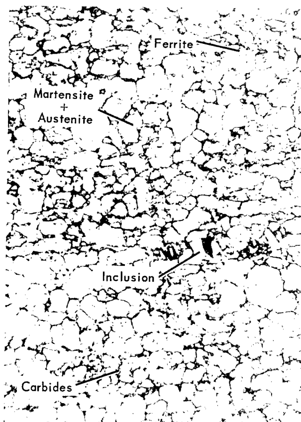
L-64-8305 Figure 11.- Microstructure of PH 15-7 Mo longitudinal specimen with zero exposure. 800x.
