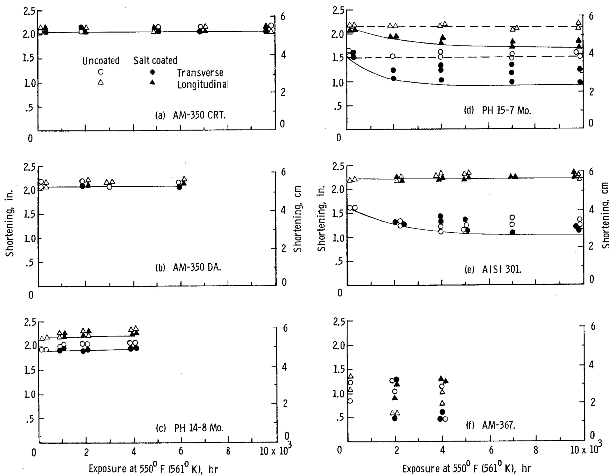
Figure 4.- Results of compression tests on specimens exposed at 550° F (561° K).
