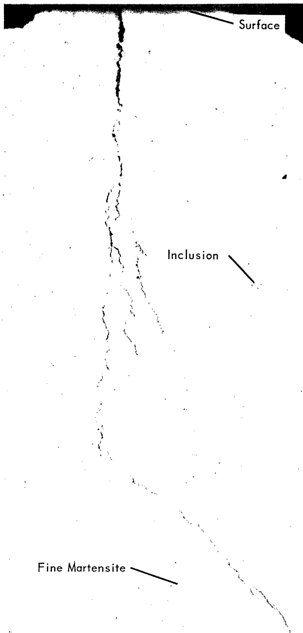
Figure 13.- Edge view of stress-corrosion cracks in AM-367 transverse specimen exposed 2760 hours outdoors. 200X.
