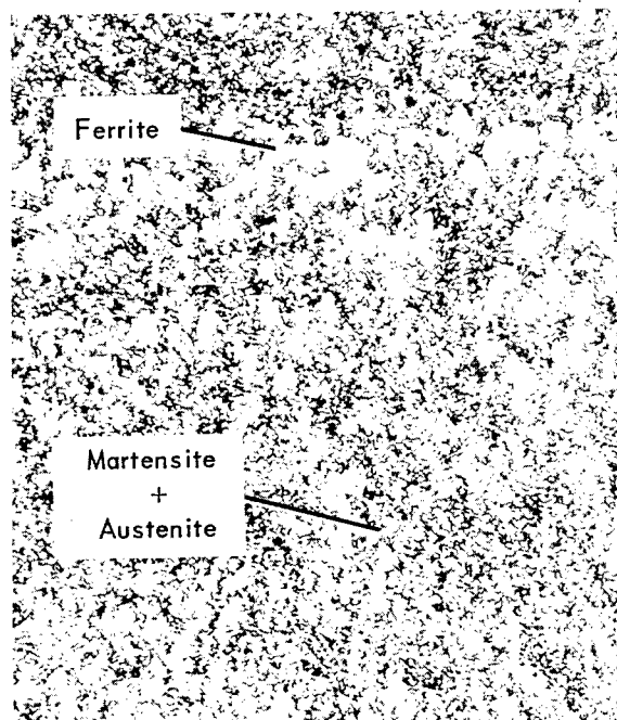
Figure 12.- Microstructure of PH 14-8 Mo longitudinal specimen with zero exposure. 800X.
