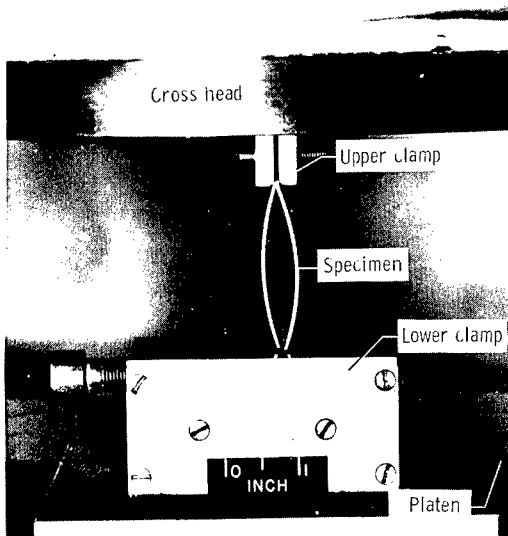
L-64-8301 Figure 2.- Clamping fixtures and compression-test apparatus.
