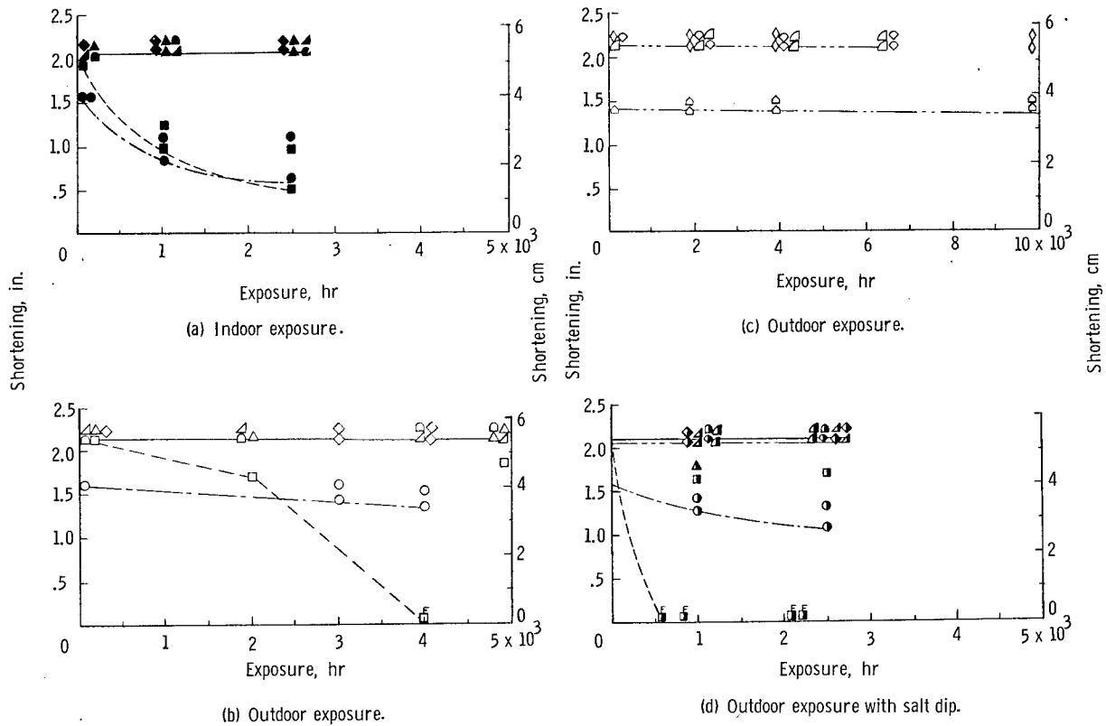
Figure 5.- Results of compression tests on specimens exposed at ambient temperatures; indoors and outdoors.
