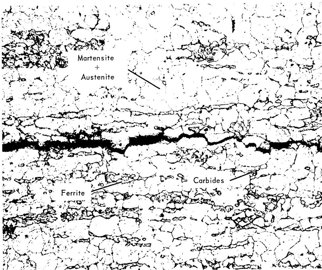
L-64-8303 Figure 9.— Top view of stress-corrosion crack in AM-350 DA longitudinal specimen exposed 500 hours at 550° F (561° K) followed by 5500 hours at room temperature. 800x.
