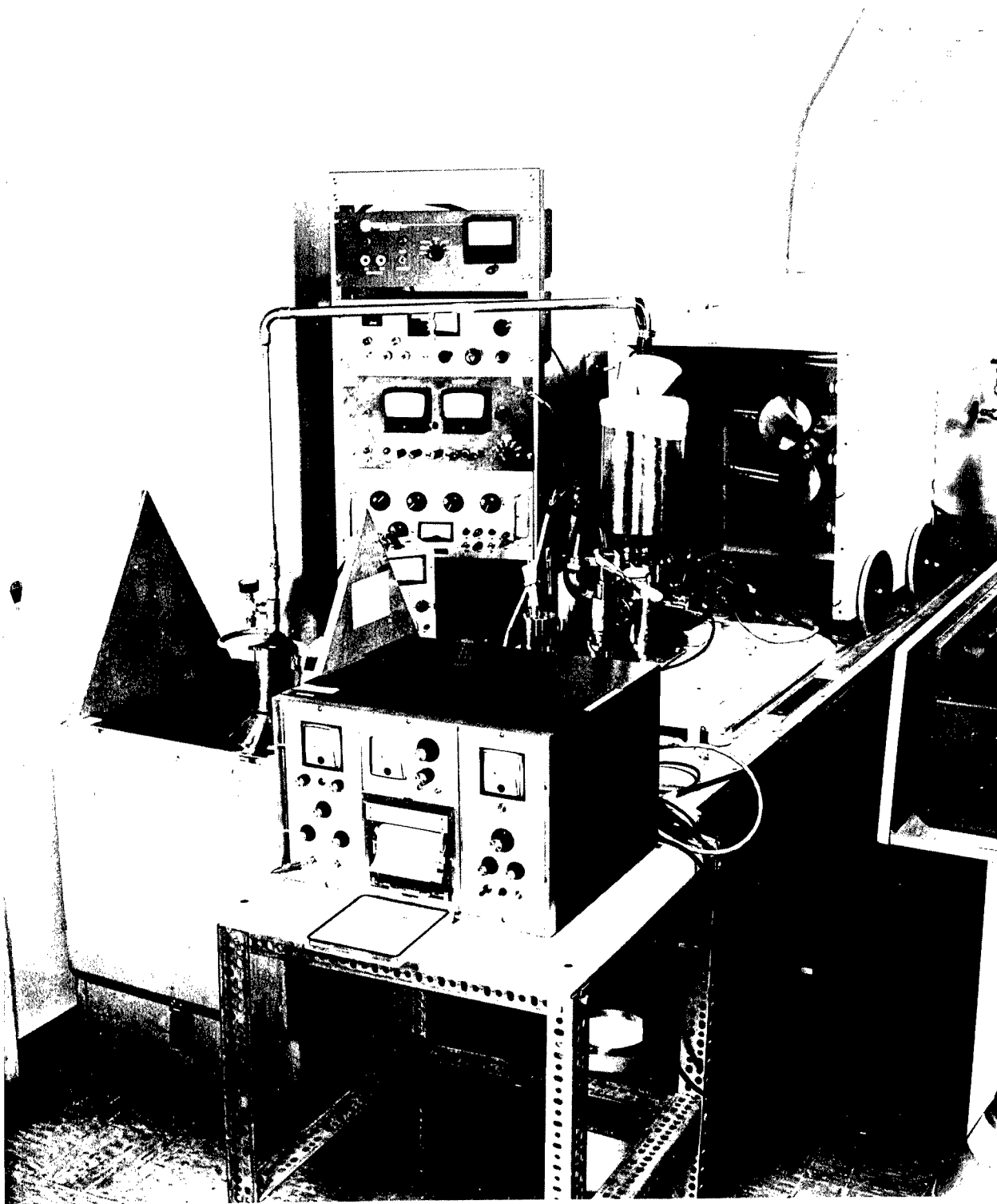
Figure 12. Photograph of cryopump-ion pump system.
