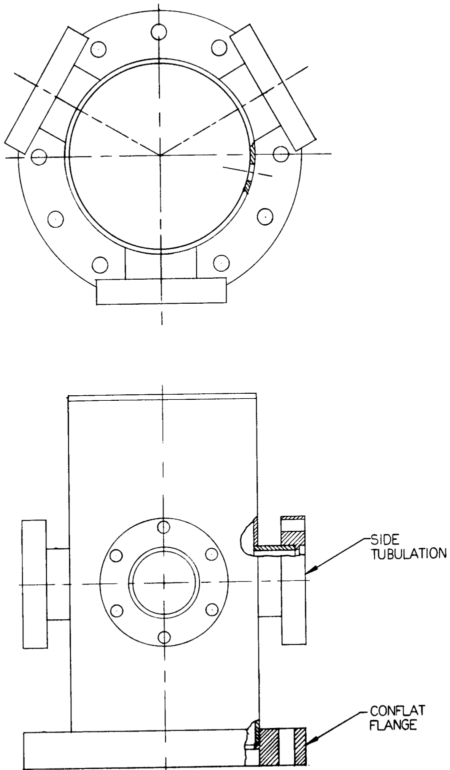
Figure 6. Test chamber.
