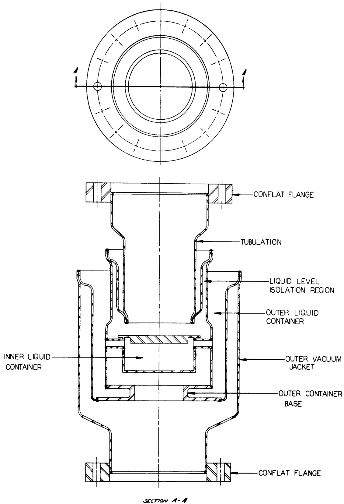
Figure 4. Non-level sensitive cold trap.
