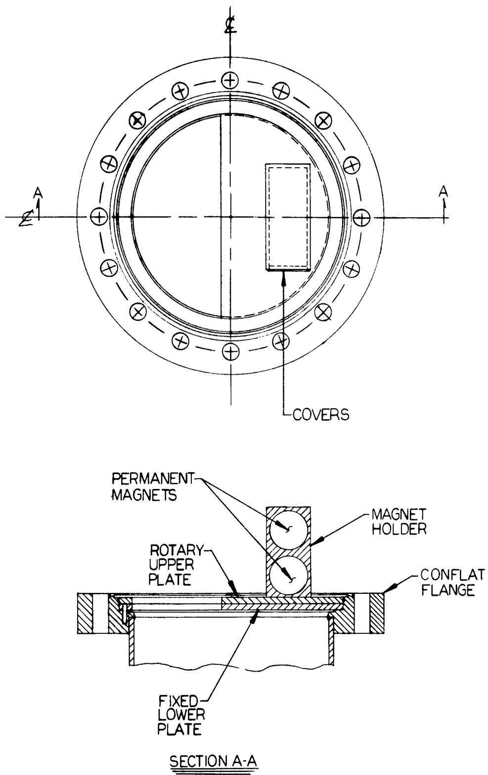
Figure 5. Vapor valve.
