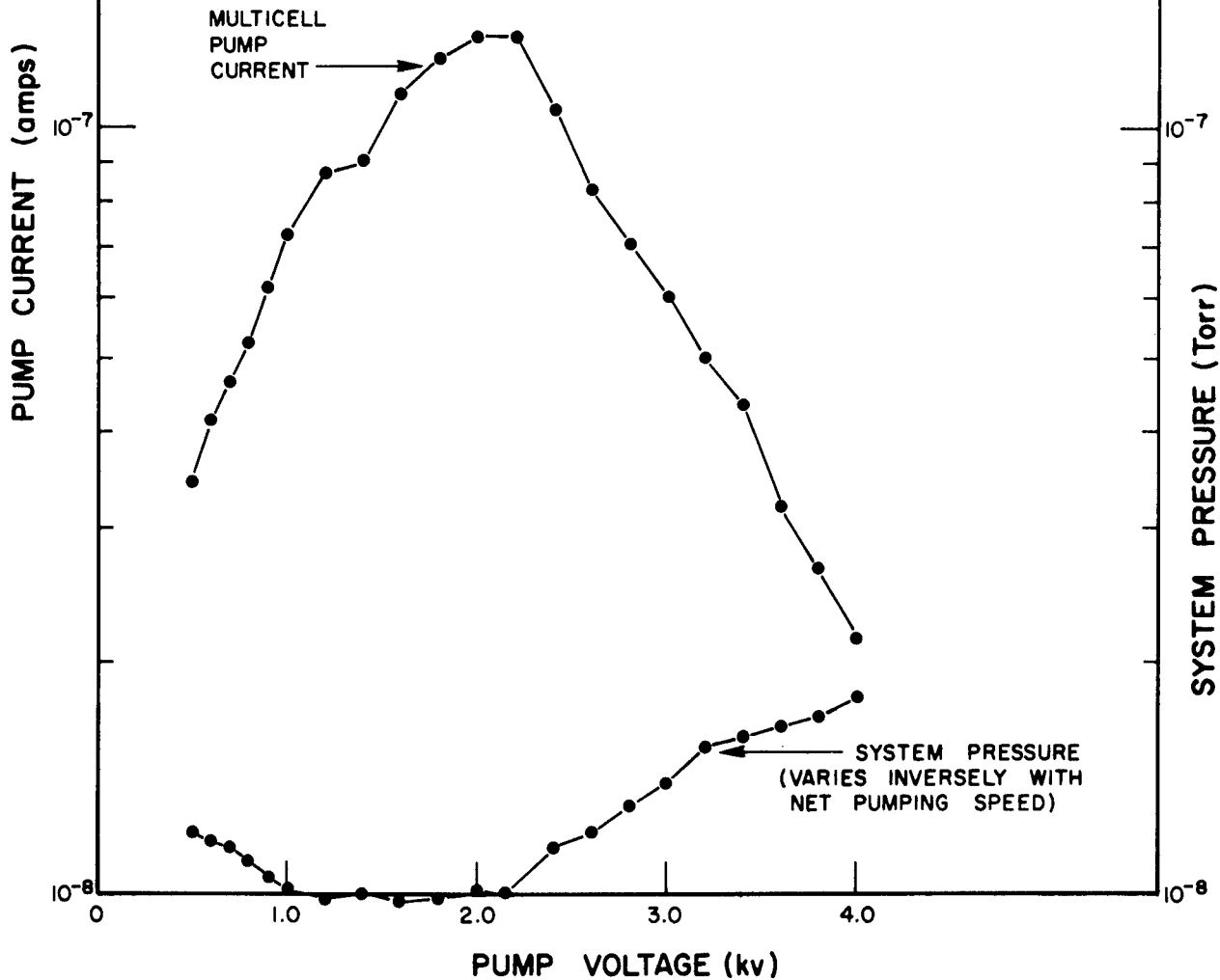
Figure 23. Current-voltage characteristic and pumping effect of the multicell magnetron type ion pump for background gas.
