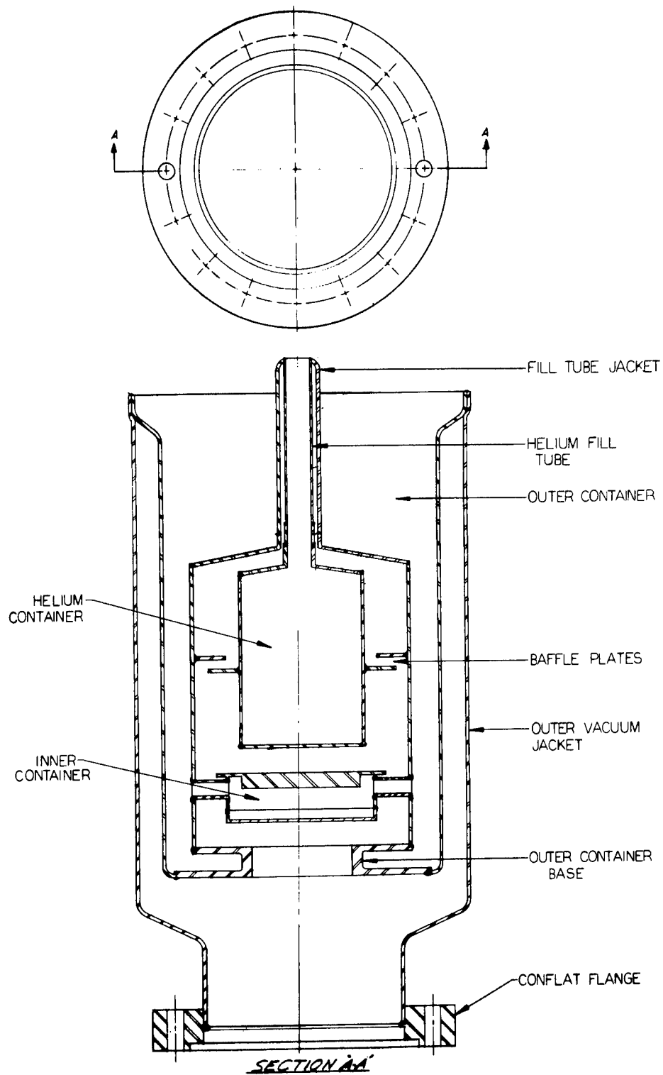
Figure 13. Liquid helium cryopump.
