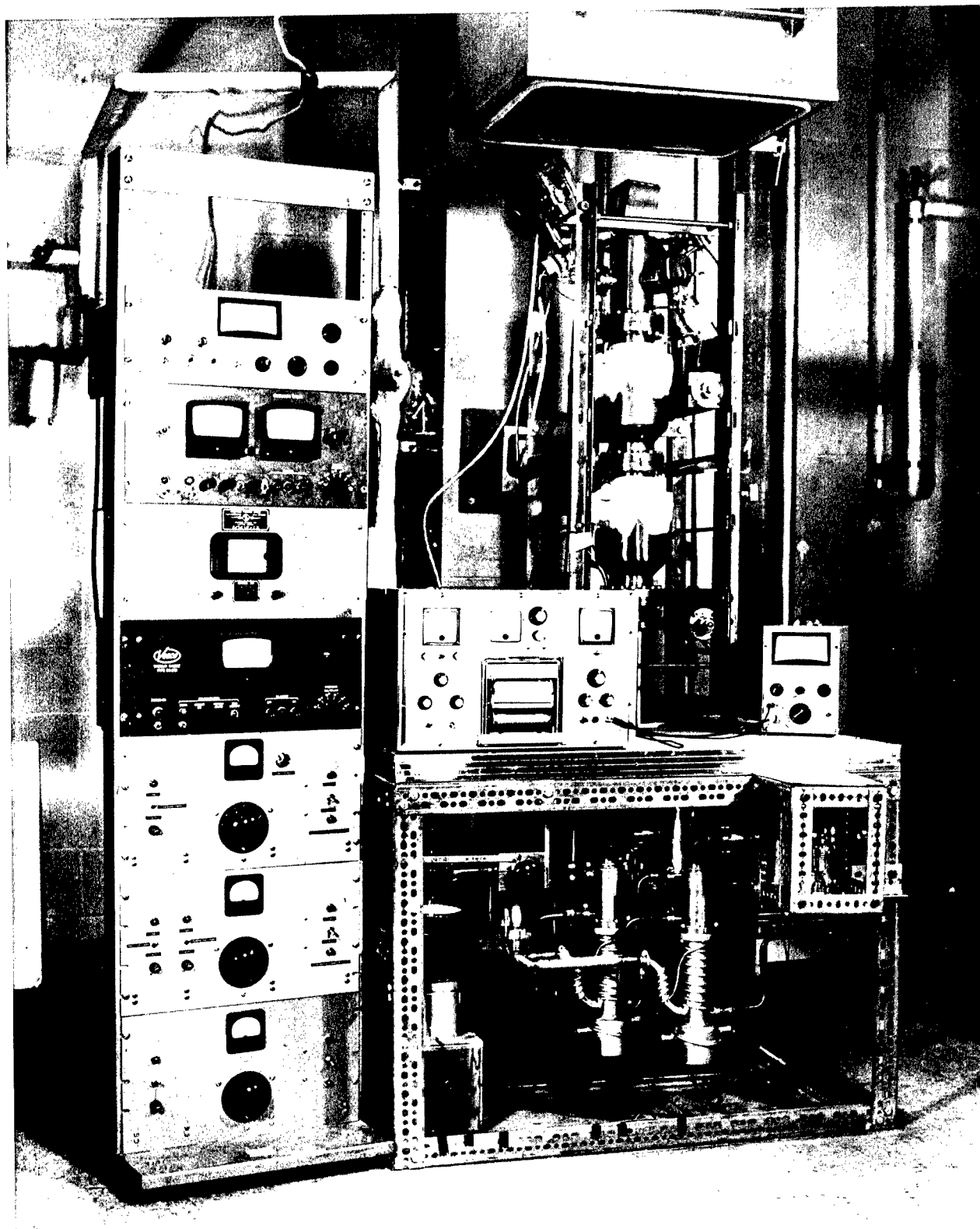
Figure 2. Photograph of mercury diffusion pump system.
