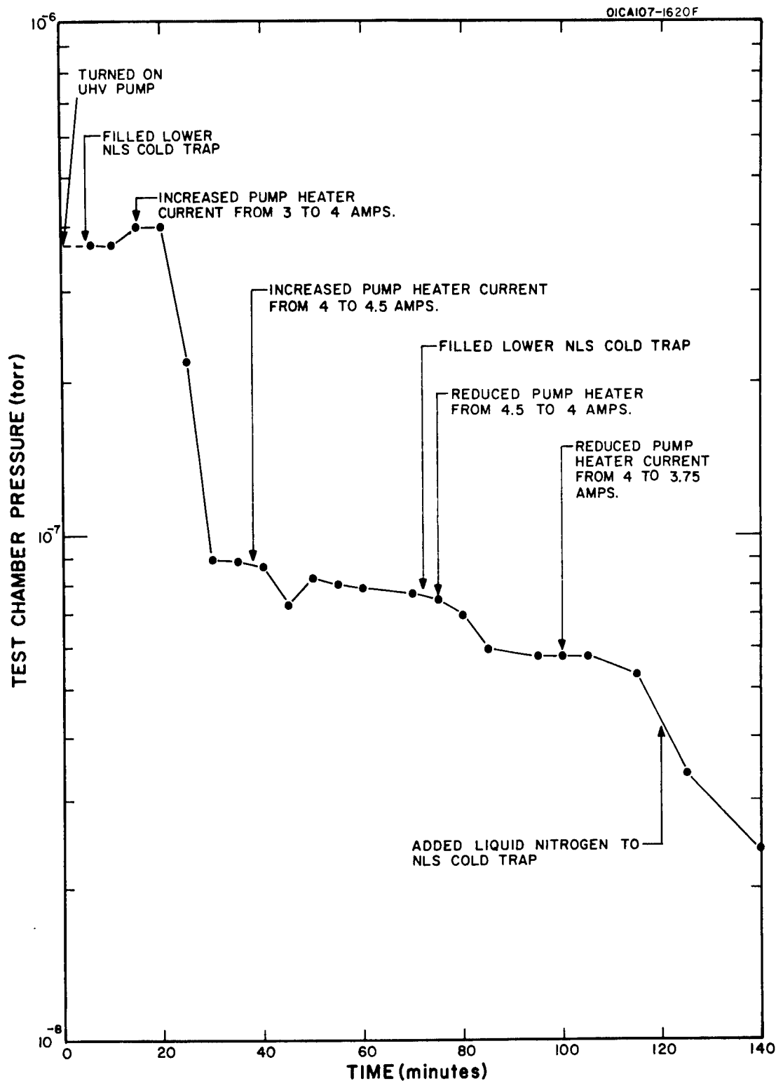
Figure 19. Time variation of pressure in the mercury diffusion pump system showing the effect of various heat inputs to the ultra high vacuum diffusion pump.
