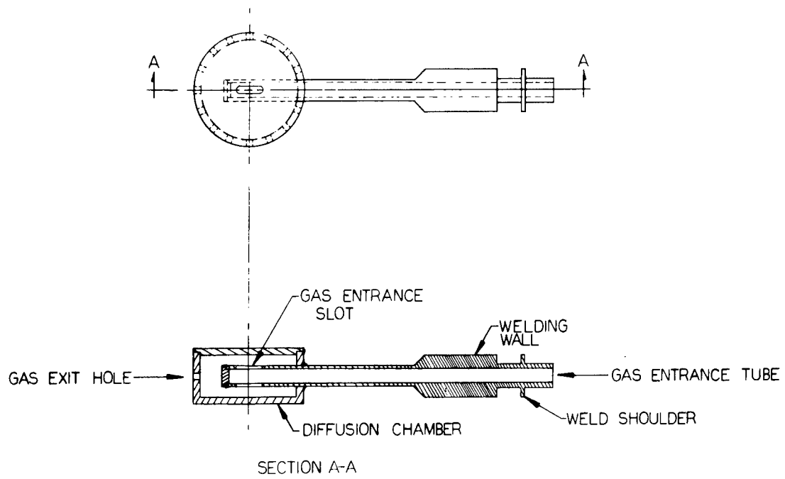
Figure 7. Gas inlet diffuser.
