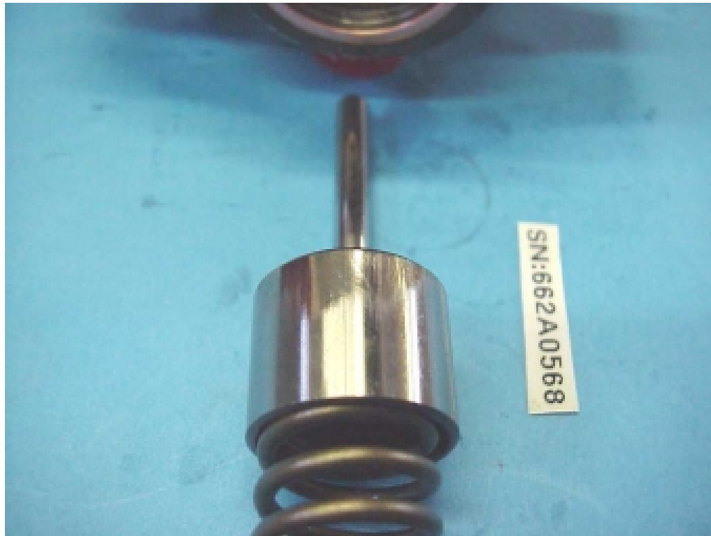
Figure B-1A. Piston to Cylinder
