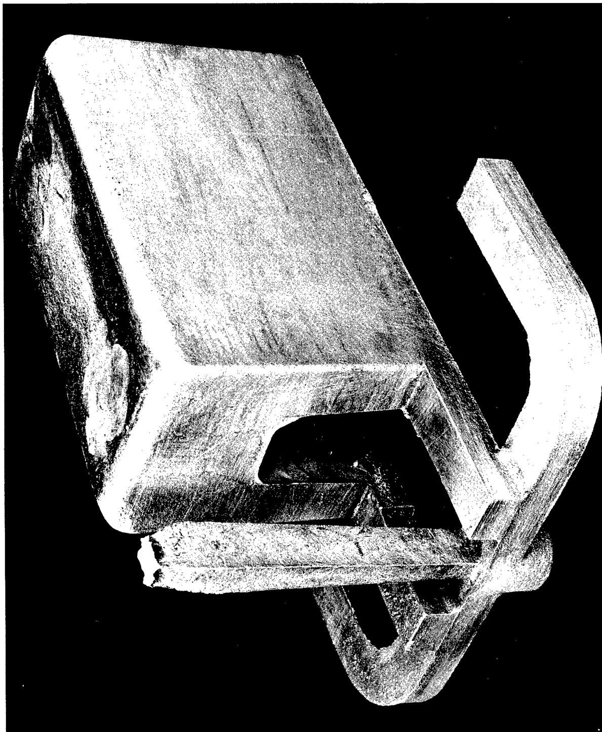
FIGURE 2. DOUBLE-LEG KEEL-BLOCK CASTING
