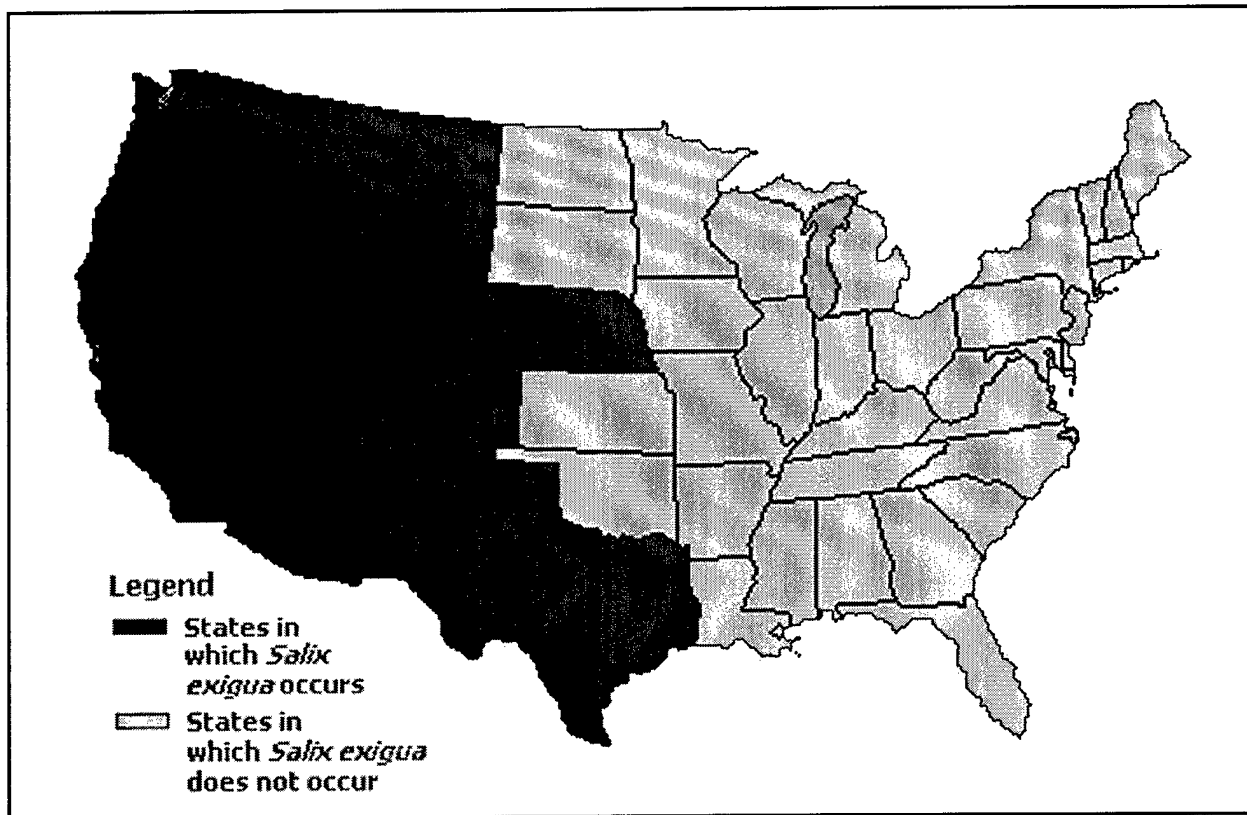
Figure 3. National distribution of Salix exigua by state (USDA 1999d)
