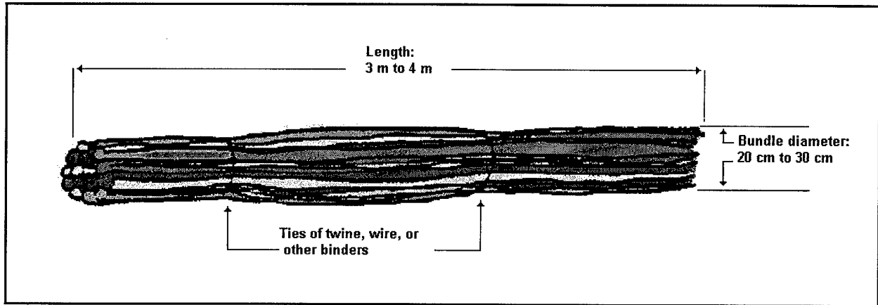
Figure 1. Schematic diagram of a fascine (wattling) bundle (U.S. Department of Agriculture 1999d)
