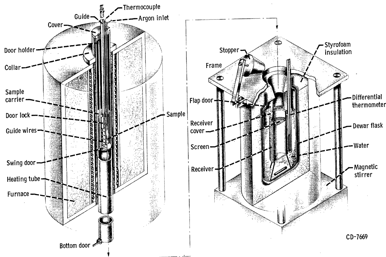
Figure 7. - Drop calorimeter.
