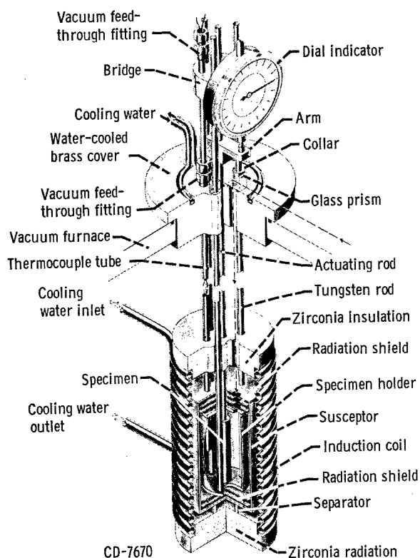
Figure 11. - Vacuum dilatometer.
