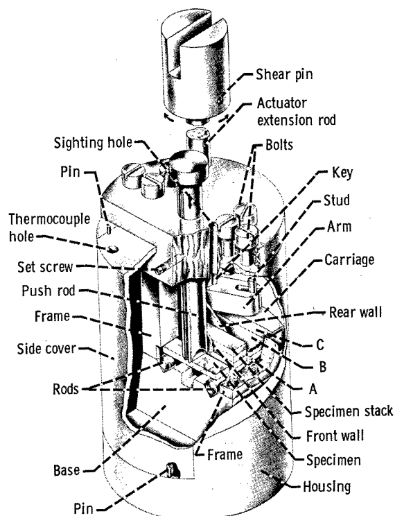
Figure 12. - Semiautomatic modulus-of-rupture tester.
