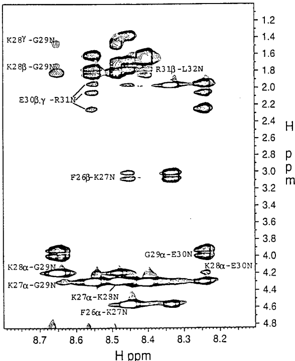
Figure 4. ROESY spectrum at pH 6.0 and 12 C. (a) the C( \alpha , \beta )H - NH region, (b) the NH - NH region. A 250 ms mixing time was used. Only the inter-residue NOEs are labelled in the spectra.
