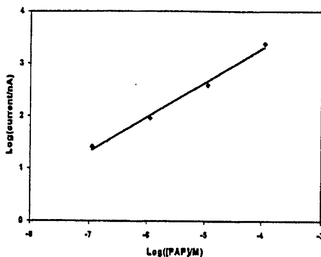
Figure VI-3: Anodic peak current Measured from the baseline current and plotted versus PAP concentration
