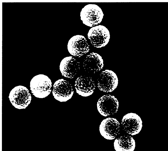
Figure III-35: Magnetic beads
