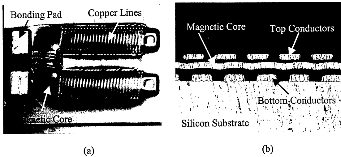
Figure III-22: Photographs of fabricated solenoid-type inductor
