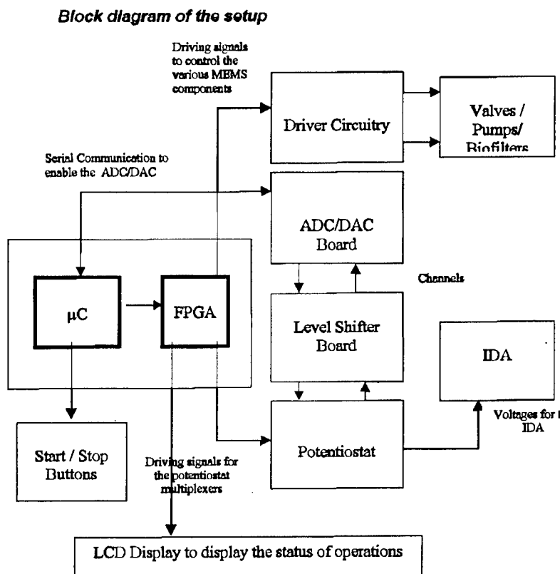
Figure III-38: Block diagram of the microcontroller based electronic system
