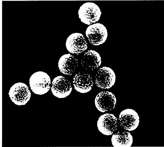
Figure VI-10: Magnetic beads
