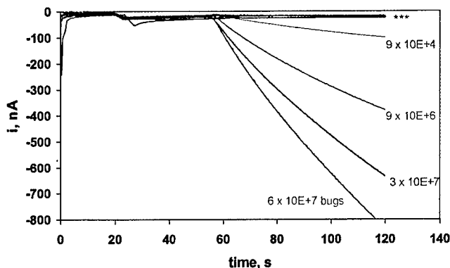
Figure III-36: RDE detection results
