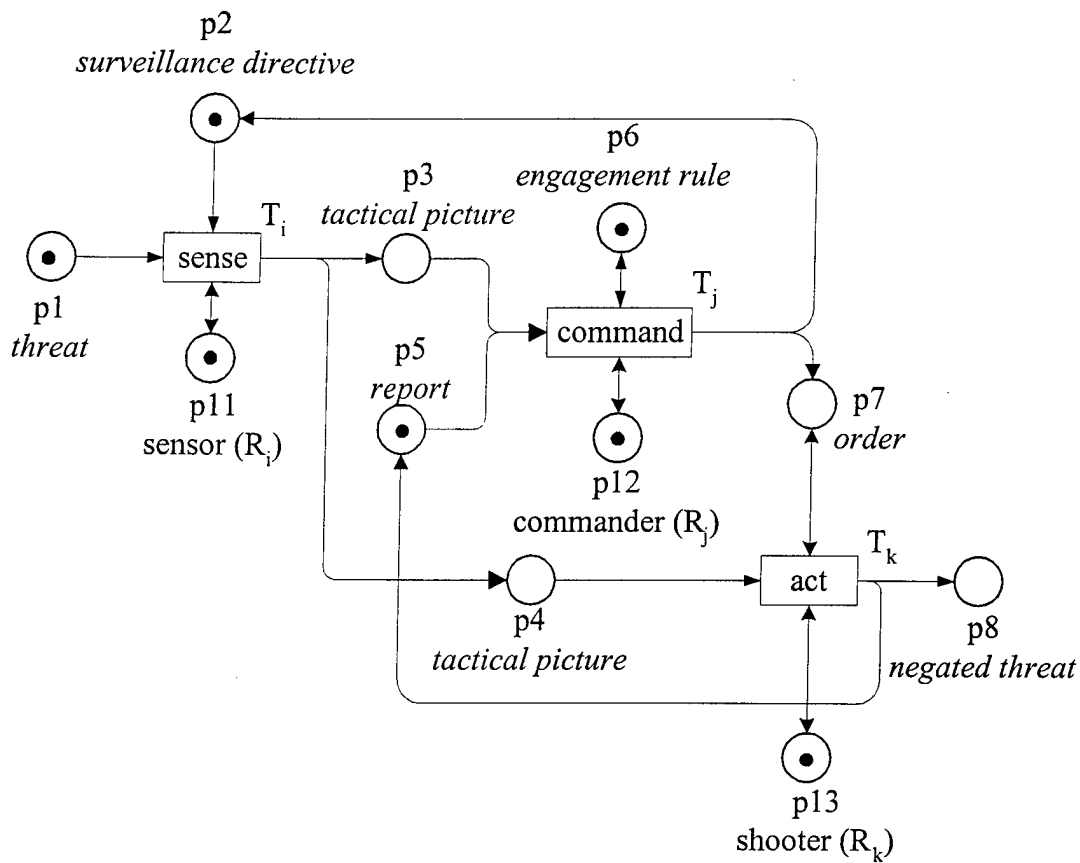
Figure 4.9 An Example of a Basic Executable Functional Model
