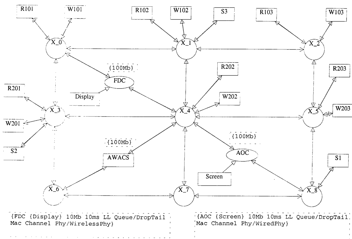
Figure 6.10 Deployment Diagram of an AAW system
