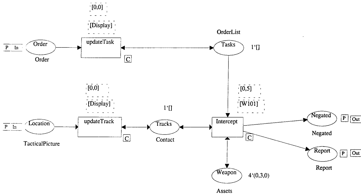
Figure B.6 Petri Net Diagram: Act
