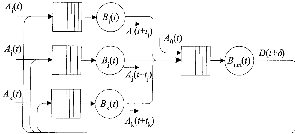
Figure 4.7 Executable Physical Model as a Queueing Net
