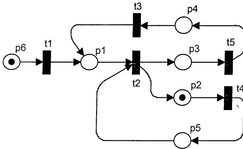
Figure 3.5 Example of Markings of Petri net
