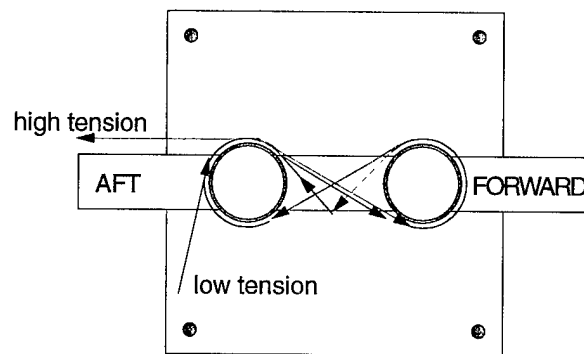
H-Bit line fair lead detail
