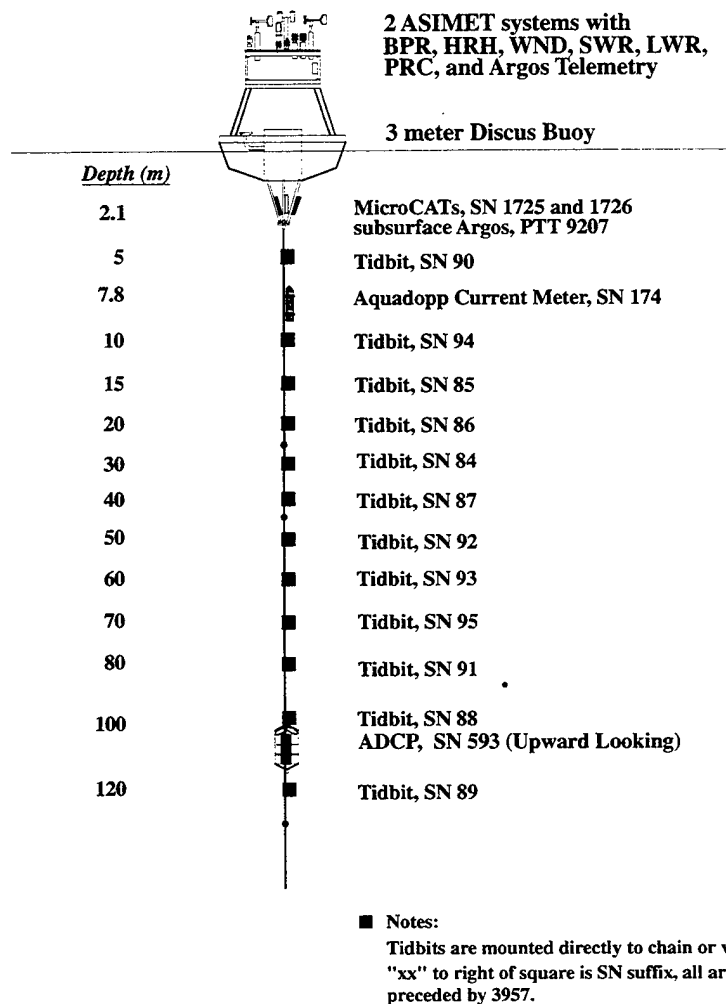
Figure 3 (cont'd): NTAS-1 mooring detail in the upper 120 m.
