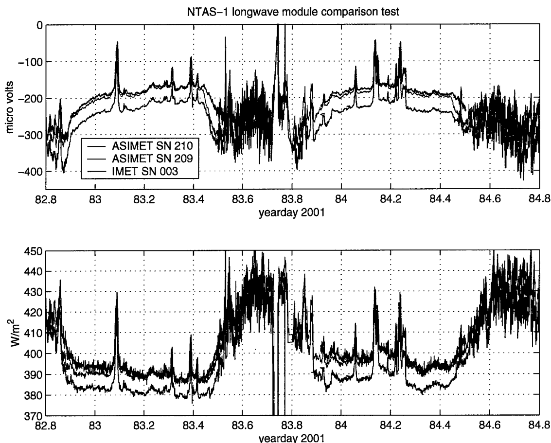
Figure 13: LWR comparison. Time series of thermopile voltage and longwave radiation from the two primary ASIMET modules and IMET LWR-003.
