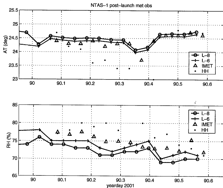
Figure 17: Post-launch comparison of air temperature (AT) and relative humidity (RH) from the two buoy systems (L-6 and L-8), the shipboard IMET system, and handheld sensors (HH).
