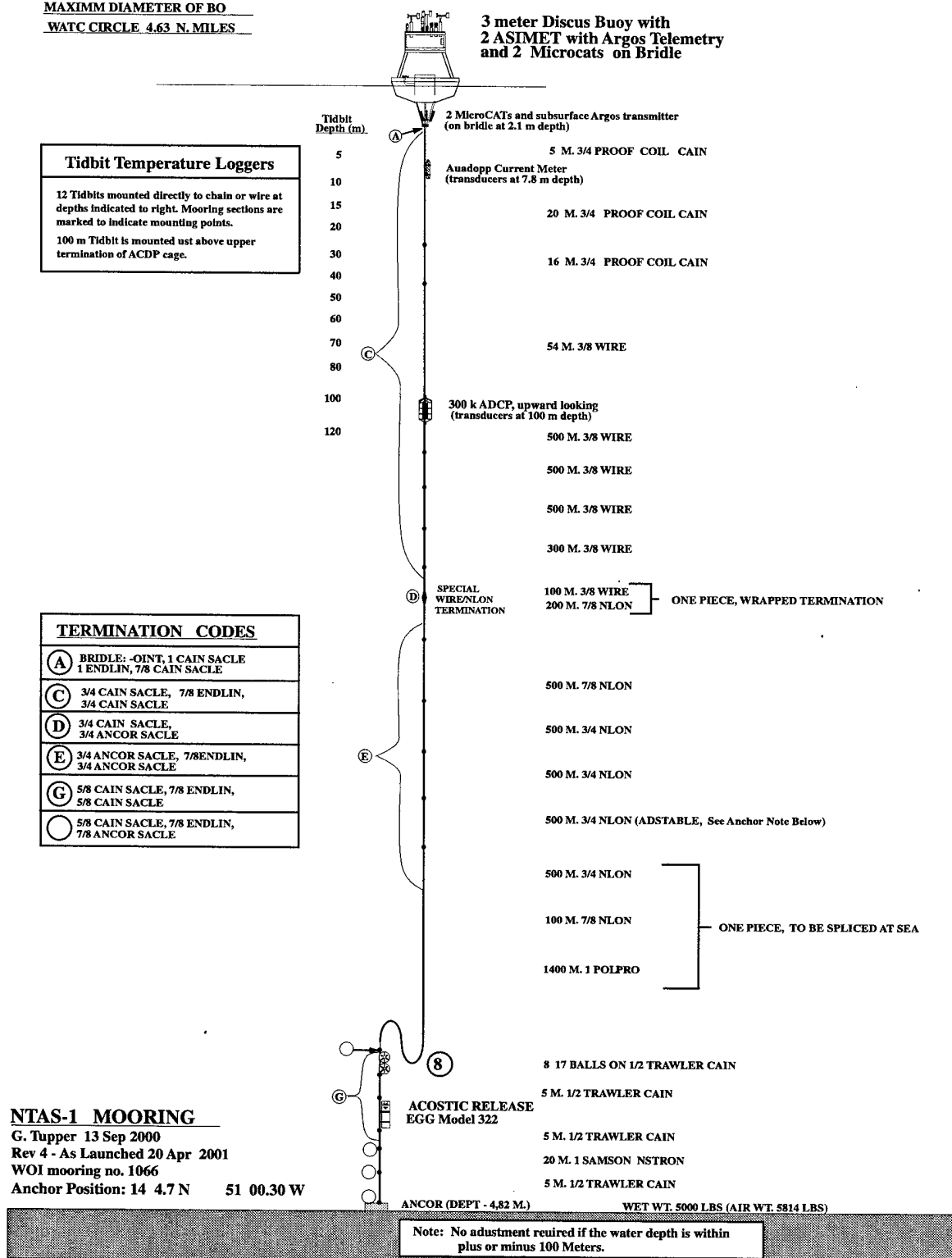
Figure 3: NTAS-1 mooring diagram.
