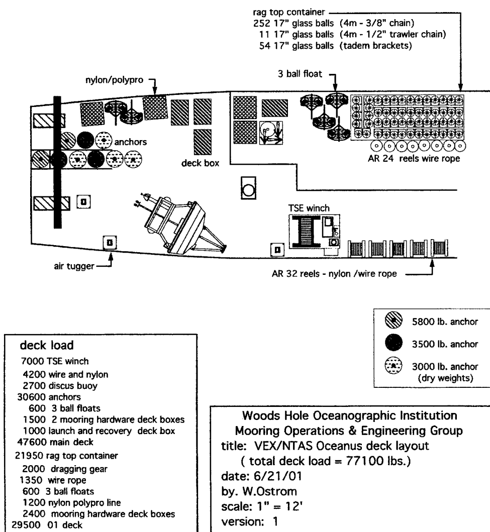
Figure 23: Basic deck equipment and deck layout for VEX and NTAS.
