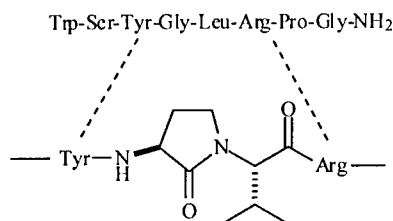
Fig. (2). Illustration of the Freidinger lactam substitution in LHRH.
