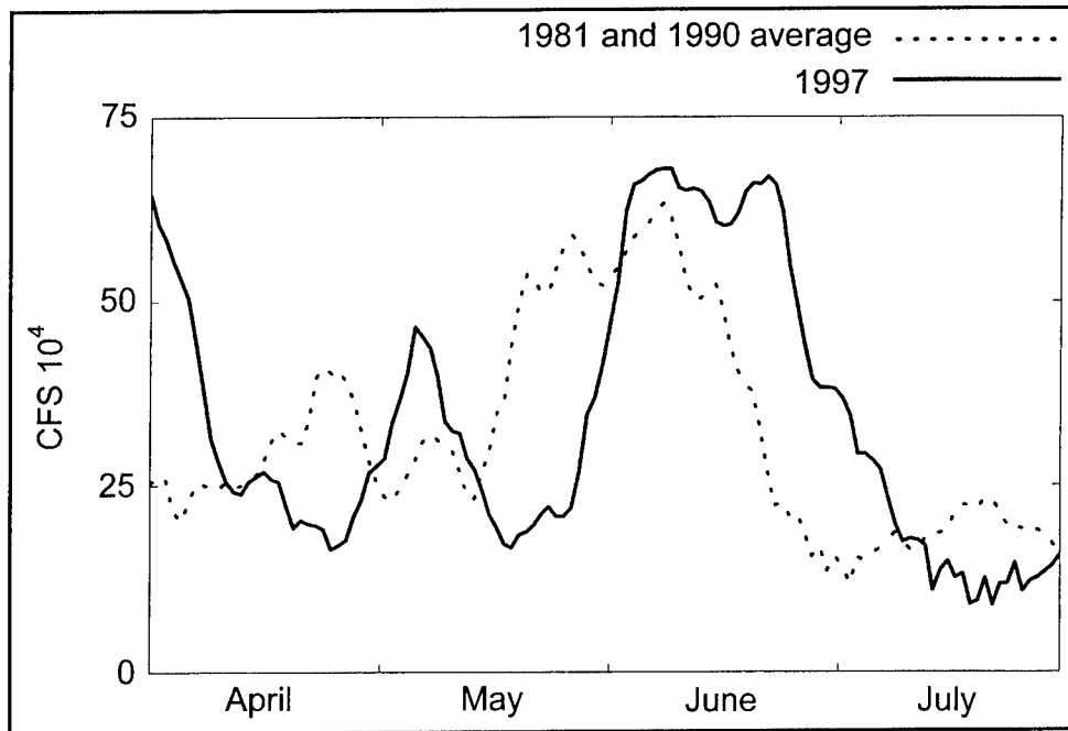
Figure 19. 1997 lower Ohio River discharge pattern
