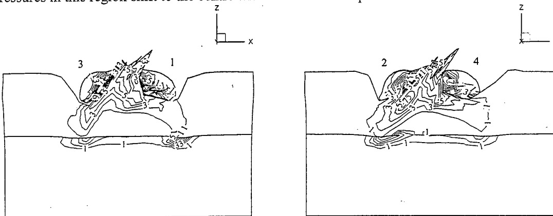
Figure 27. Distribution of pressure isolines in cross sections ZX (a) and ZY (b) on simultaneous impact. Material 1 is the shell material. t=6\mu\text{sec} . 1 - 1GPa, 2 - 2GPa, ..., 10 - 10GPa.
