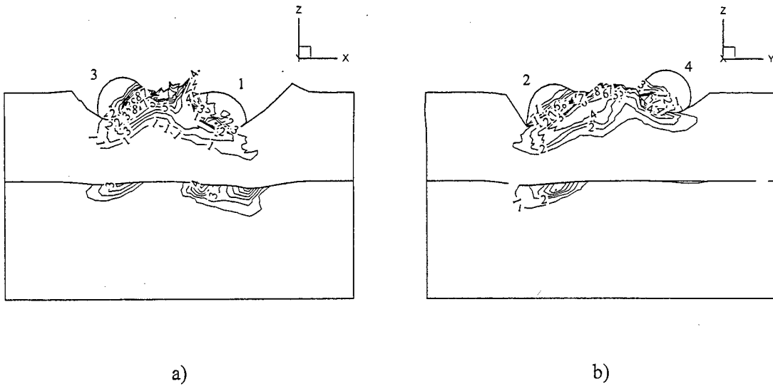
Figure 30. Distribution of pressure isolines in cross sections ZX (a) and ZY (b) on different in time impact. Material 2 is the shell material. t=6\mu\text{sec} . 1 - 1GPa, 2 - 2GPa, ..., 10 - 10GPa.
