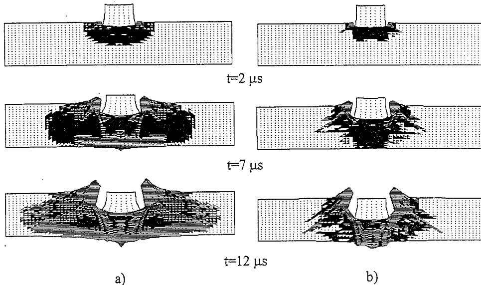
Figure 3. Evolution destruction areas in isotropic (a) and transtropic (b) barrier. v_0=1000 m/s, \alpha=0^\circ , h=19 mm, m=10 g.
