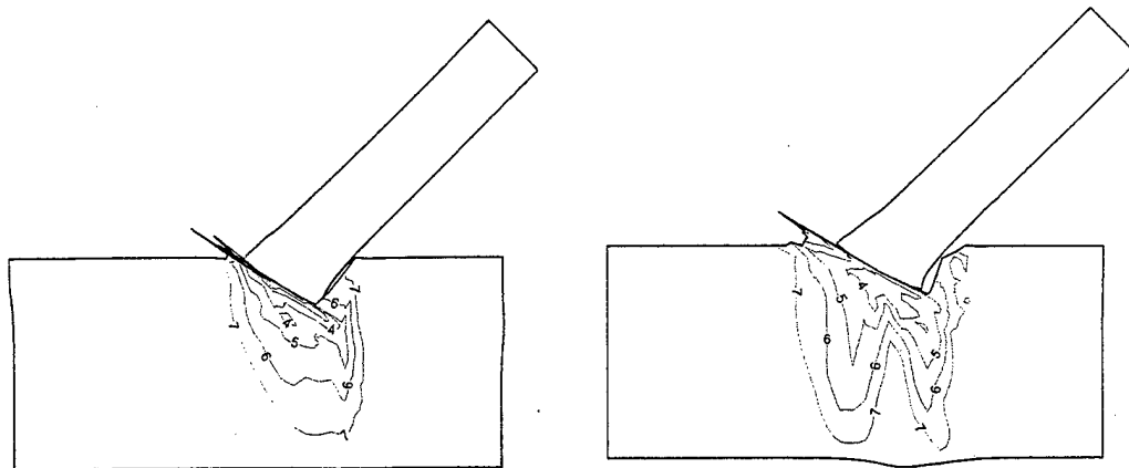
Figure 19. Isolines \sigma_z in section ZOX at the moment of time t=12\mu\text{sec} . v_0=1000 m/sec, \alpha=45^\circ , where 1 - 2GPa, 2 - 1.7 GPa, 7 - 0.2GPa. The material 1 - at the left, a material 2 - on the right.
