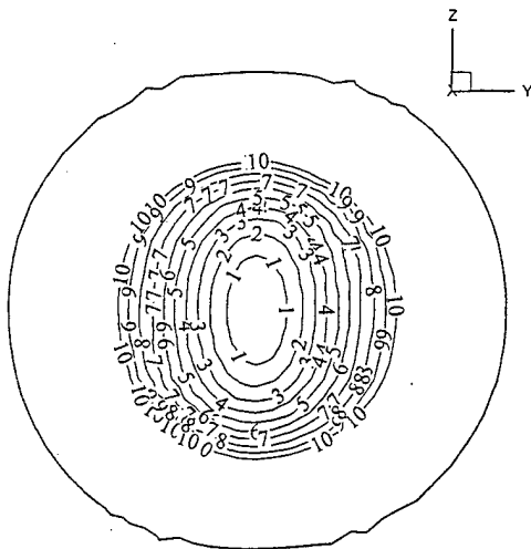
Figure 40. Distribution of isolines of stress \sigma_x . t=1.2\mu\text{sec.} 1 - -3GPa, 2 - -2.8GPa, 3 - -2.6GPa, 4 - -2.4GPa, ..., 10 - -1.2GPa.
