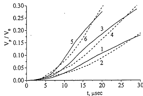
Figure 15. The change in time of relative amount of the material, being failed at e_{kk} > 0 . 1, 3, 5 – in material 1; 2, 4, 6 – in material 2 at v_0=700 \text{ m/sec} , 1000 \text{ m/sec} , and 1500 \text{ m/sec} , respectively.
