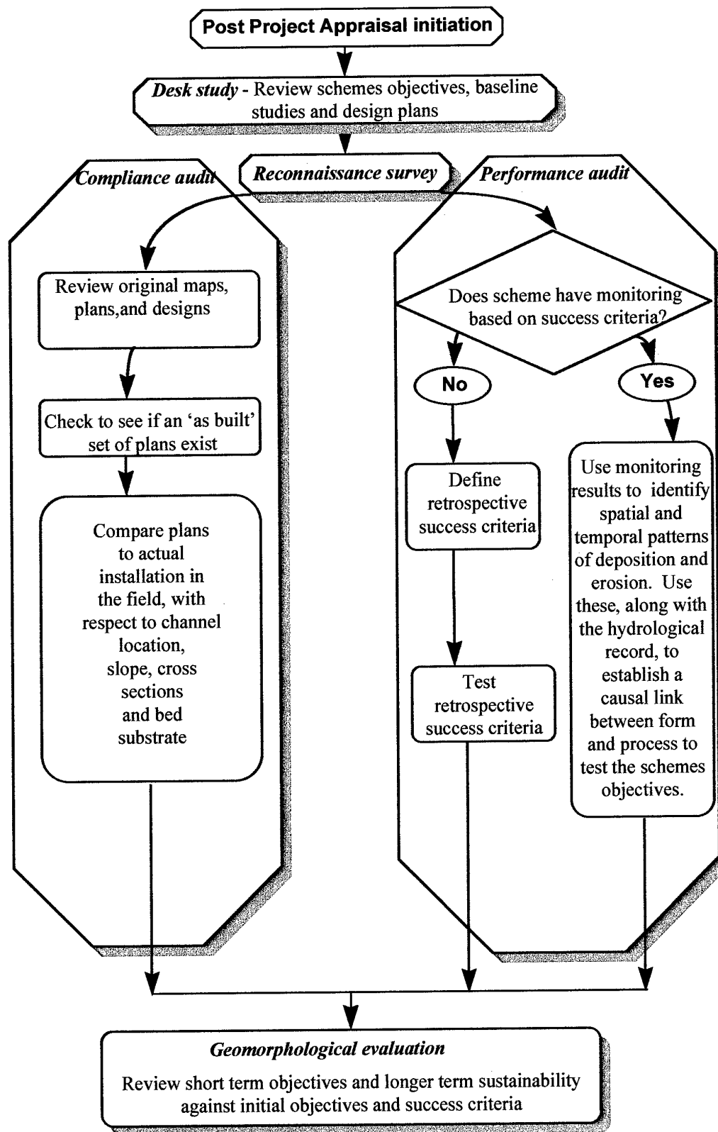
Figure 9: Geomorphic Post-Project Appraisal Procedure (adapted from Skinner, 1999)
