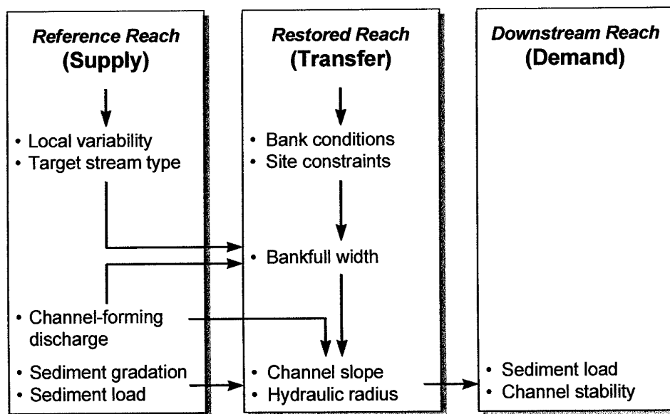
Figure 3 : Sediment Continuity in the fluvial system (from Soar et al. , 2001)
