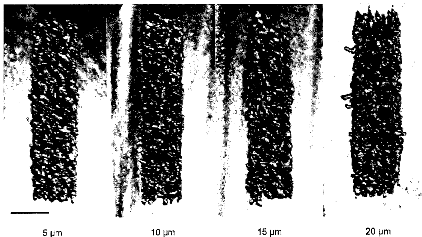
Fig. 7.17 Views of intrastromal bubble layers produced by 25 \mu\text{J} , 45 ps pulses with 5-20 \mu\text{m} lateral distance between the application sites of subsequent laser pulses. The scale is 250 \mu\text{m} .
