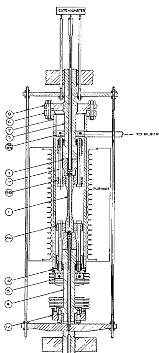
Figure 11-2. - Furnace, vacuum chamber, and specimen holder assembly for Mo-0.5 Ti fatigue tests.
