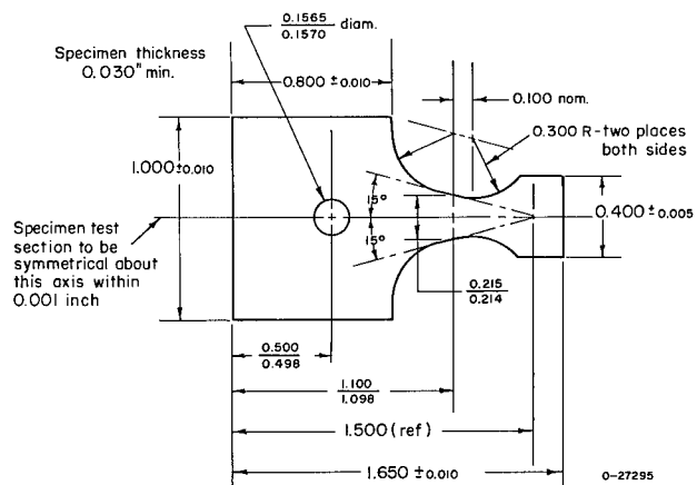
Figure I-1. - Nb-1Zr fatigue specimen.
