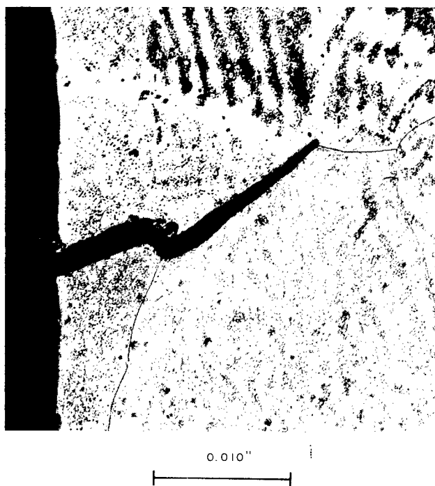
Figure 9. - Areas of intergranular attack observed in the transverse section of Cb-1Zr capsule weld exposed to liquid potassium for 1000 hours at 2000° F. Etchant: 60% glycerine, 20% HNO 3 , 20% HF.
