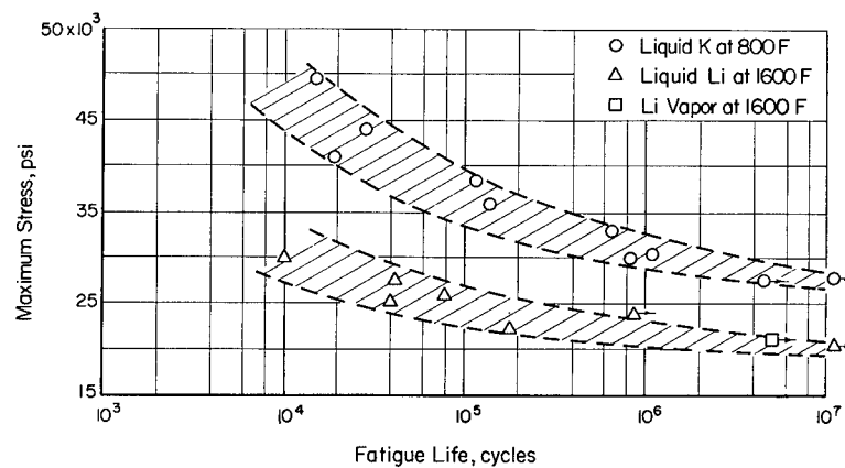
Figure I-4. - Results of reversed-bending fatigue tests on Cb-1Zr in liquid potassium at 800 F and liquid lithium at 1600 F.
