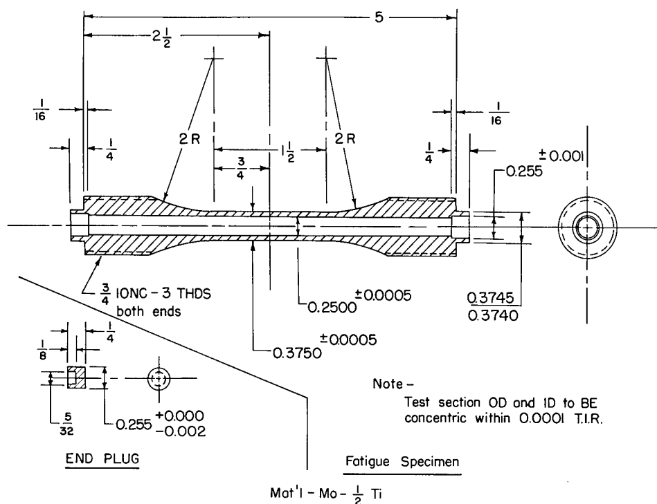
Figure 11-1. - Dynamic creep specimen for modified Ivy machine.
