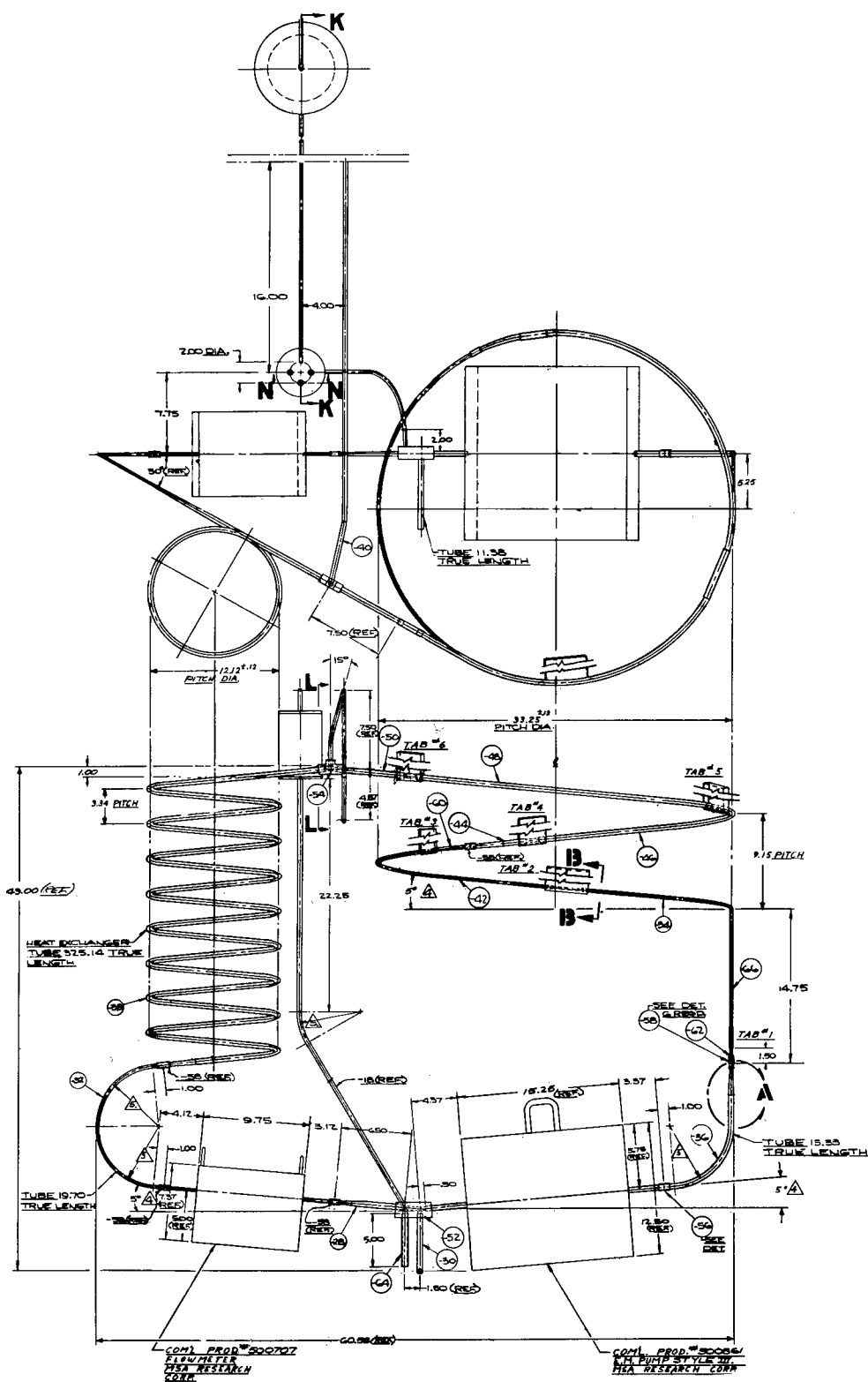
Figure 1. - Dynamic test loop for liquid rubidium.
