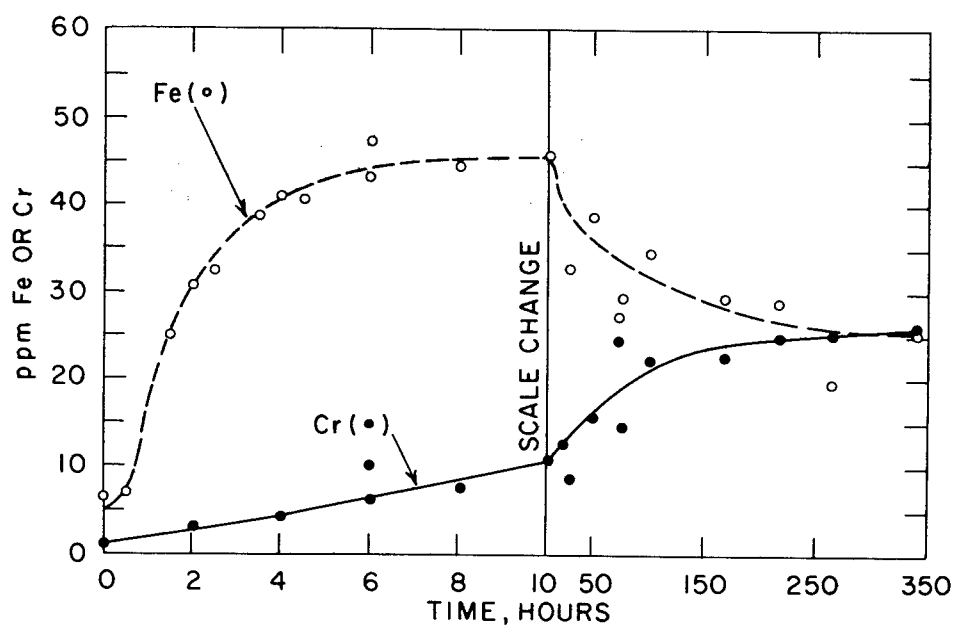
Figure 2-3. - Concentration of Fe and Cr in Bi contained in an 410 steel crucible as a function of time at 600° C. Crucible had been filled with Bi at 410° C where solubilities are negligible. Data at zero time are from a sample taken at 410° C immediately before the temperature was raised.
