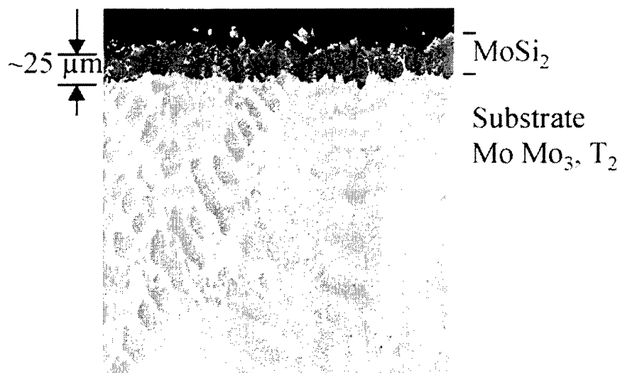
Figure 26. Microstructure of the As-Deposited MoSi 2 Coating on Mo-10Si-13B Using a Simple CVD Process
