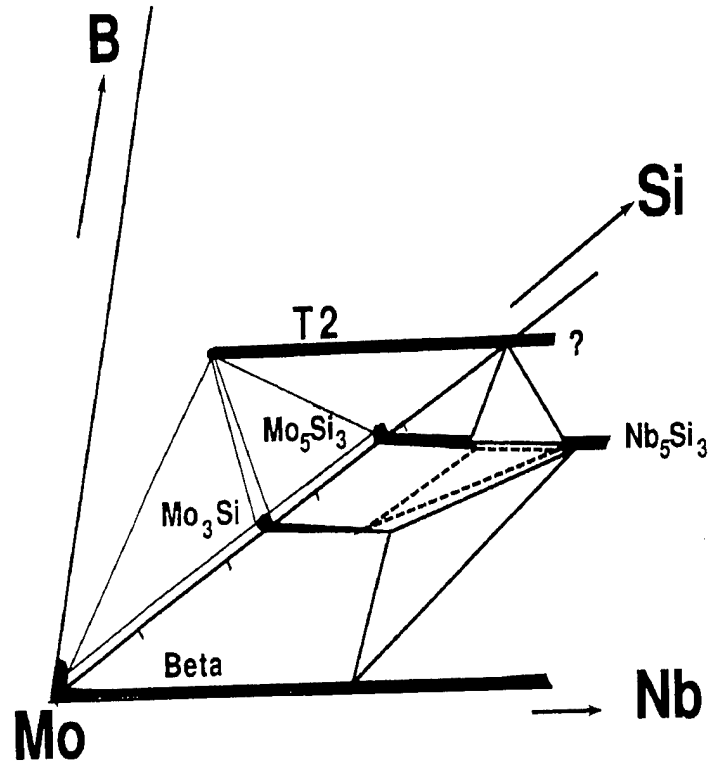
Figure 5. Possible Phase Diagram at 1400 °C for Mo-Rich Corner of the Mo-Nb-Si-B System
