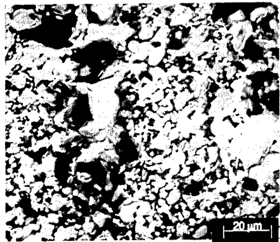
Figure 25. Cross Sectional SEM Microphotographs Showing Thick, Multiphased Oxide Scale for 48 hr Exposure at 1300 °C
