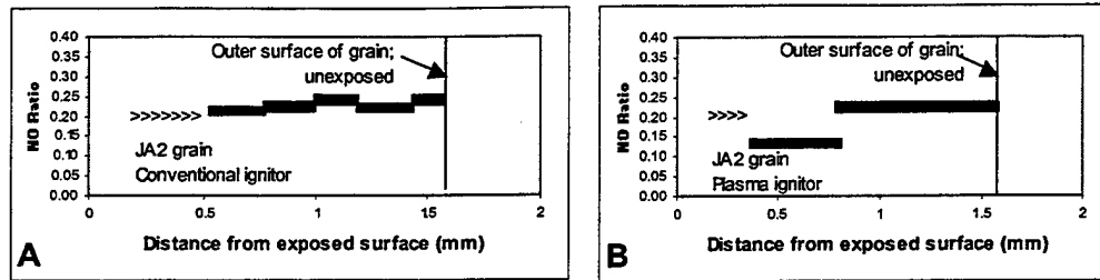
Figure 7. NO ratios for JA2 propellant grains. Nominal sample thickness is 1.55 mm. Filled boxes represent NO level in slice whose thickness is the length of the box; ">>>" indicates regression from surface.
