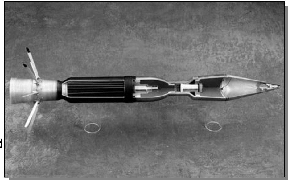
SMAW-D with Follow Through Grenade
