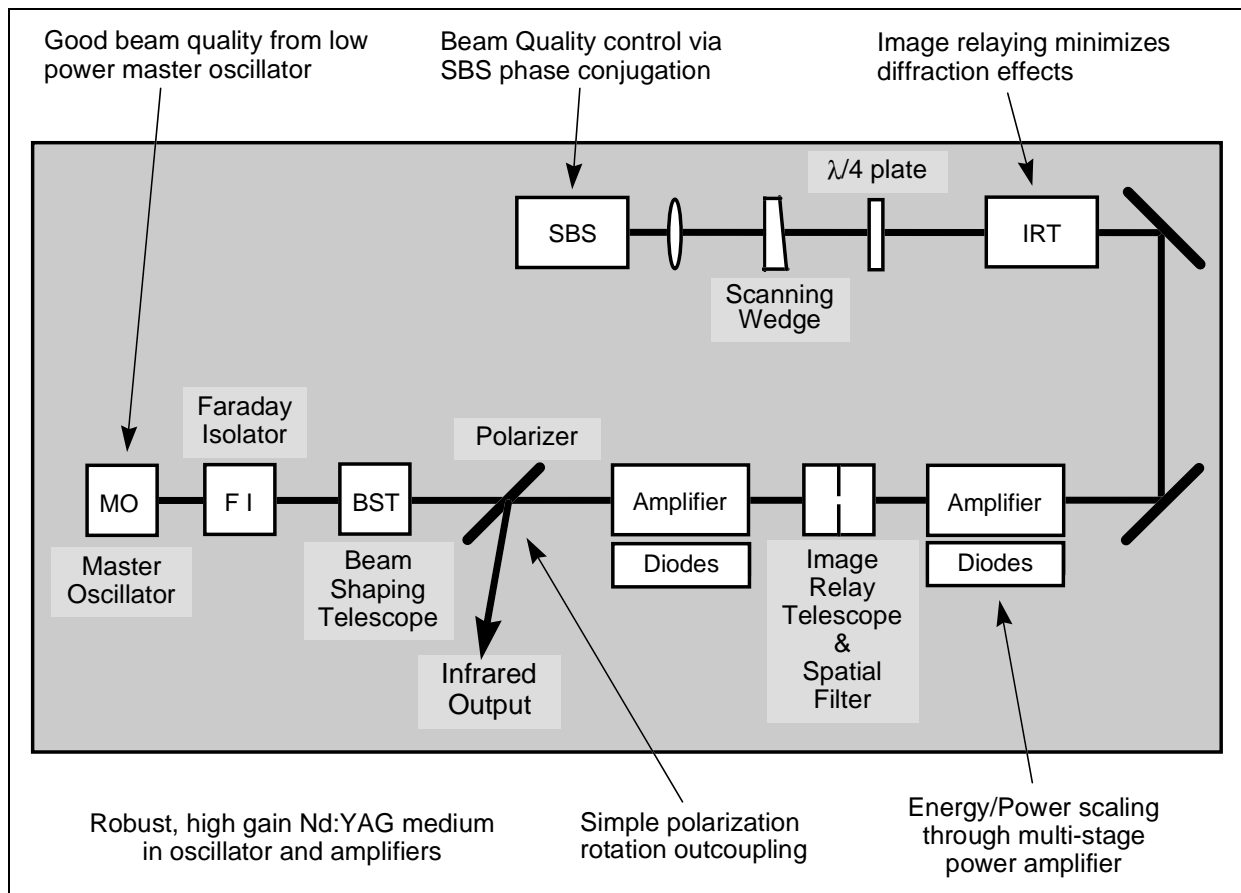
Figure 2: TRW Active Tracker Laser (ATLAS) brassboard optical schematic.
