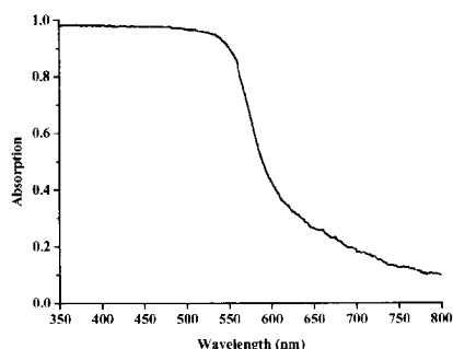
Figure 6. UV-Visible optical absorption spectrum of hematite nanorod-array.
