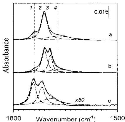
Figure 1. IRS spectra for \text{MUA-Au}_{5\text{-nm}} (a), \text{MUA-Au}_{2\text{-nm}} (b), and MUA monolayer (c). The dashed lines represent spectral deconvolution of the \nu_{\text{C=O}}(\text{CO}_2\text{H}) spectral envelope.
