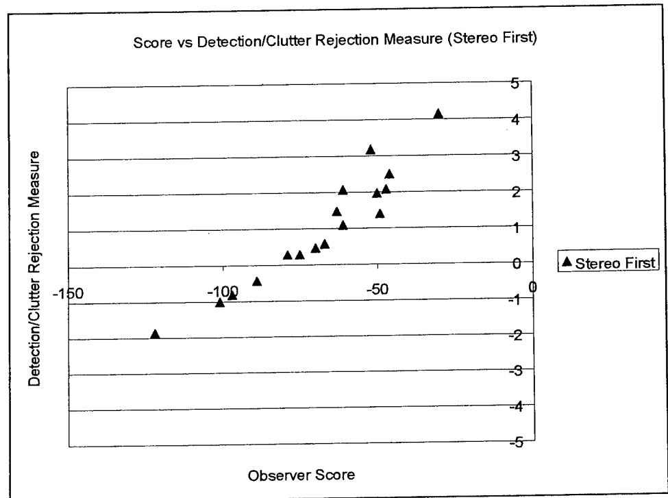
Figure A-43. Plot of observer score versus detection/clutter rejection measure for the stereo vision first test.
