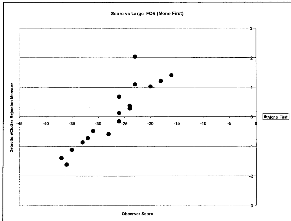
Figure a-45. Plot of observer score versus rejection/clutter rejection measure for large FOV mono first test.
