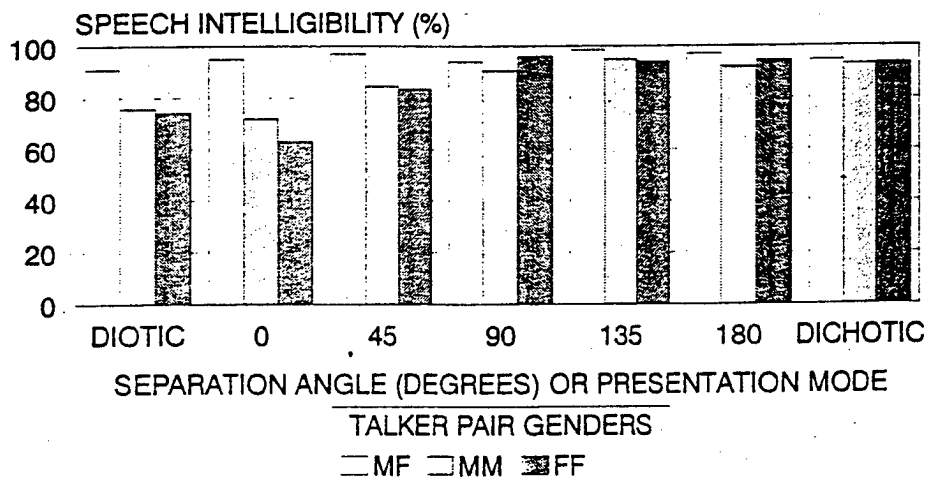
FIG. 7. Speech intelligibility for diotic, dichotic, and directional presentations of two talkers in quiet (65 dB SPL of ambient noise). Speech intelligibility was measured by the CRM with talker presentation levels set to most comfortable levels.
