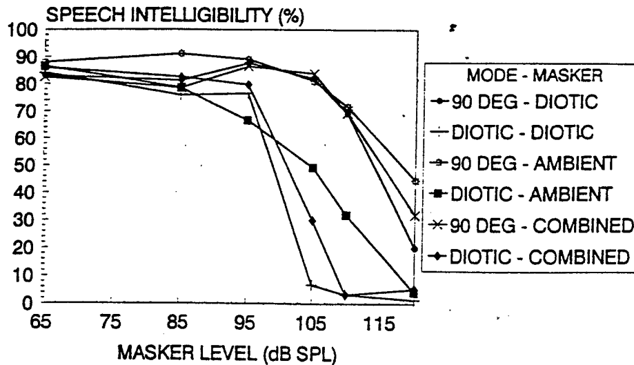
FIG. 4. Speech intelligibility of male and female speech versus masking noise level. Speech intelligibility was measured by the CRM at fixed presentation levels.
