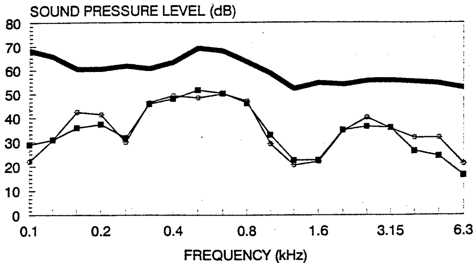
FIG. 3. Long-term average (32 s) of female speech (■), female speech (*), and 105 dB SPL noise (thick line) spectra.
