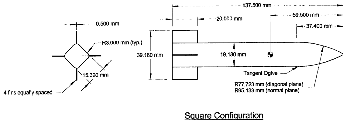
Figure 23. Square Body Cross Section Configuration
