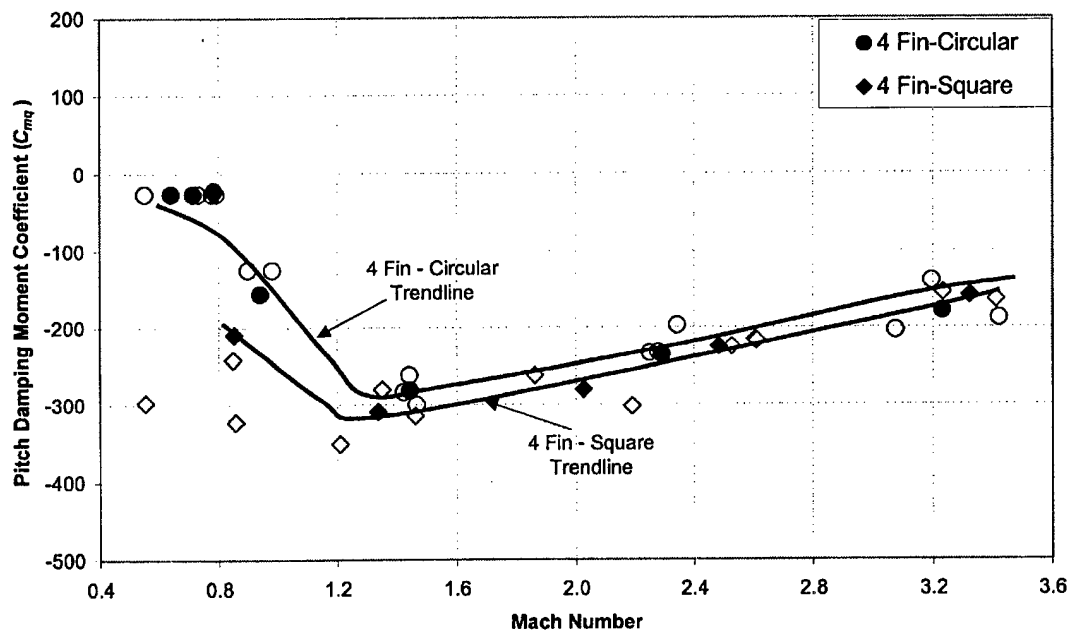
Figure 27. Pitch Moment Damping Coefficient versus Mach Number – Square Cross Section Configuration
