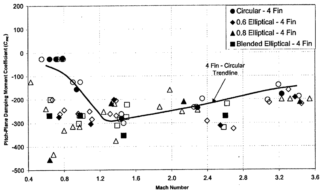
Figure 17. Pitch-Plane (Alpha-Plane) Damping Moment Coefficient versus Mach Number - Elliptic Cross Section Configurations
