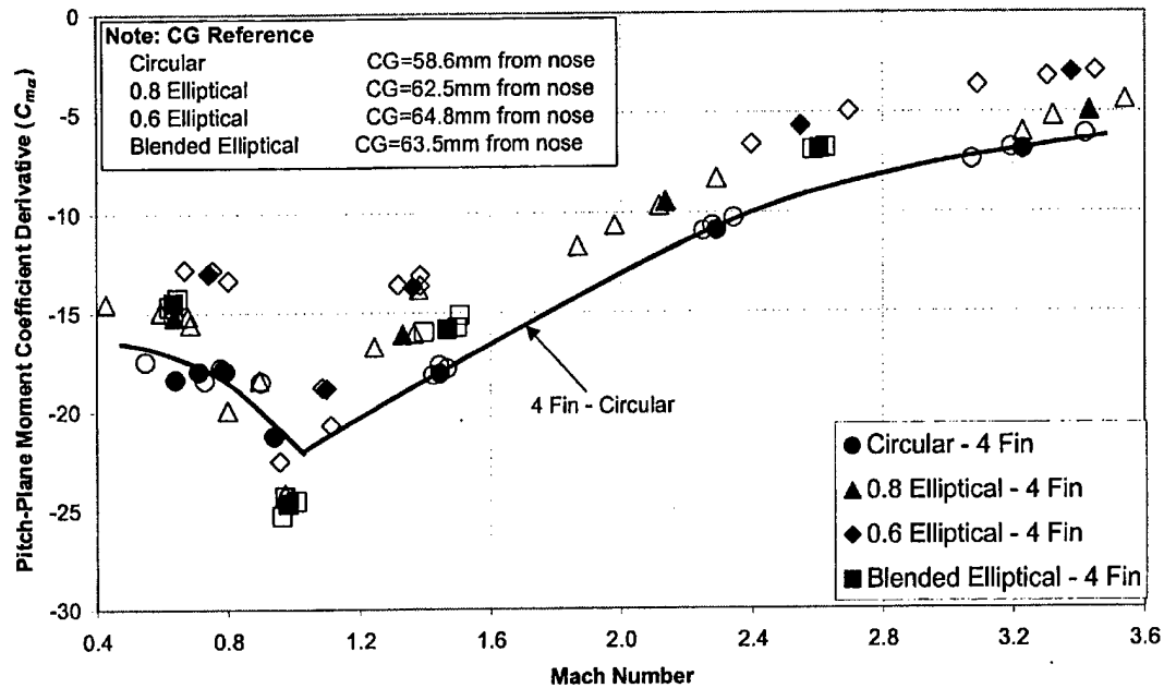
Figure 13. Pitch-Plane (Alpha-Plane) Moment Coefficient Derivative versus Mach Number - Elliptic Cross Section Configurations
