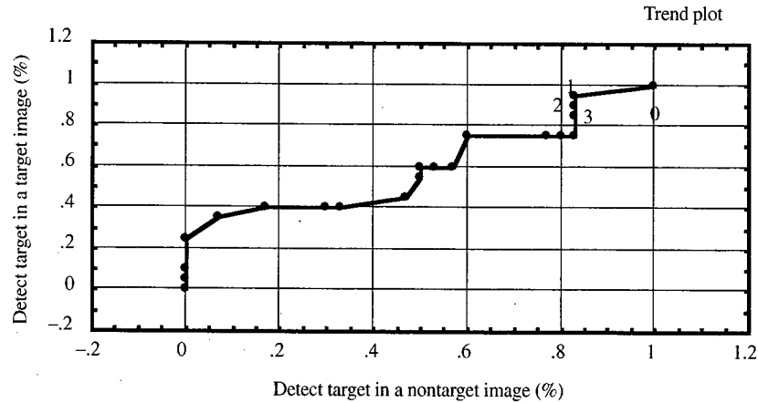
Figure 10. Worst ROC.
