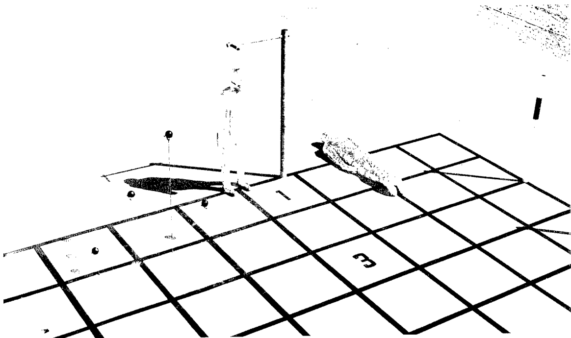
Fig. 2.1—Views from camera tower showing dummies and spheres. (a) Shot 1, without aluminum foil. (b) Shot 2, with foil.
