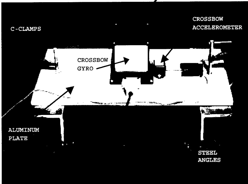
Figure 2. Sensor and secured mounting plate.
