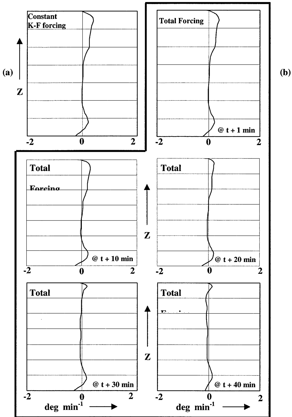
Fig. 19. (a) Vertical profile of continuous thermal forcing as dictated by the K-F convective parameterization scheme. Units are deg min -1 . (b) Time series of the atmospheric heating rate at a given time resulting from the cumulative effect of the thermal forcing applied in (a) and atmospheric response. t is the initiation time of thermal forcing by the K-F scheme.
