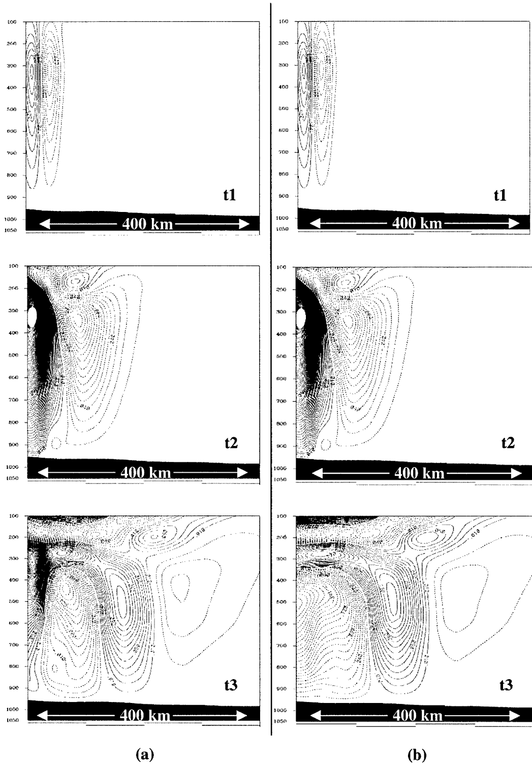
Fig. 14. Vertical cross-section of vertical velocity extending from thermal forcing at the left edge. The vertical scale is measured in hPa. The contour interval is 5 \text{ cm s}^{-1} . (a) Persistent heat source. (b) Heat source removed after 45 minutes (t2).
